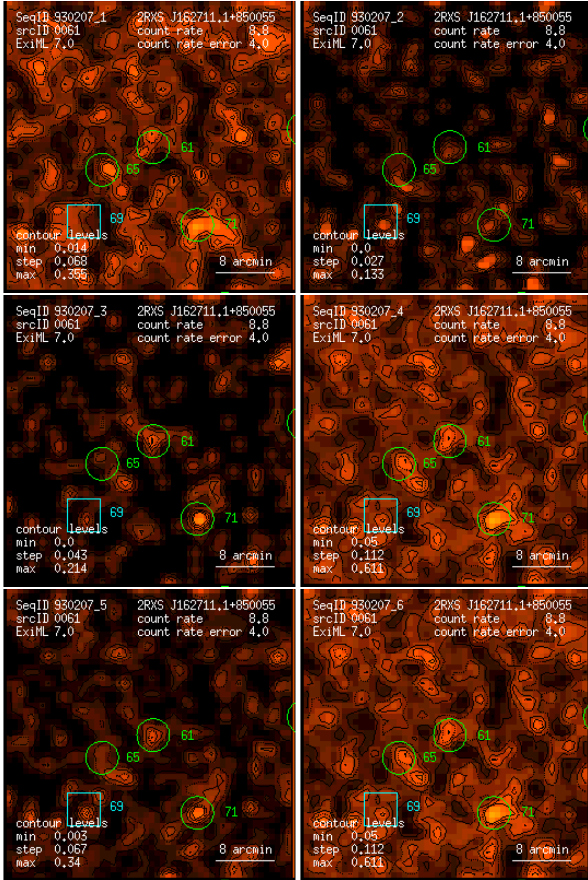
Figure 61: RASS 930207: detection 0061: band rate images, Gaussian filter: (1) PSPC channels 11 – 41, (2) 52 – 90, (3) 91 – 201, (4) 11 – 235, (5) 52 – 201, (6) 11 – 201. Broad band rates in counts/ks. Band rate contour levels in counts/ks/arcmin 2 .
