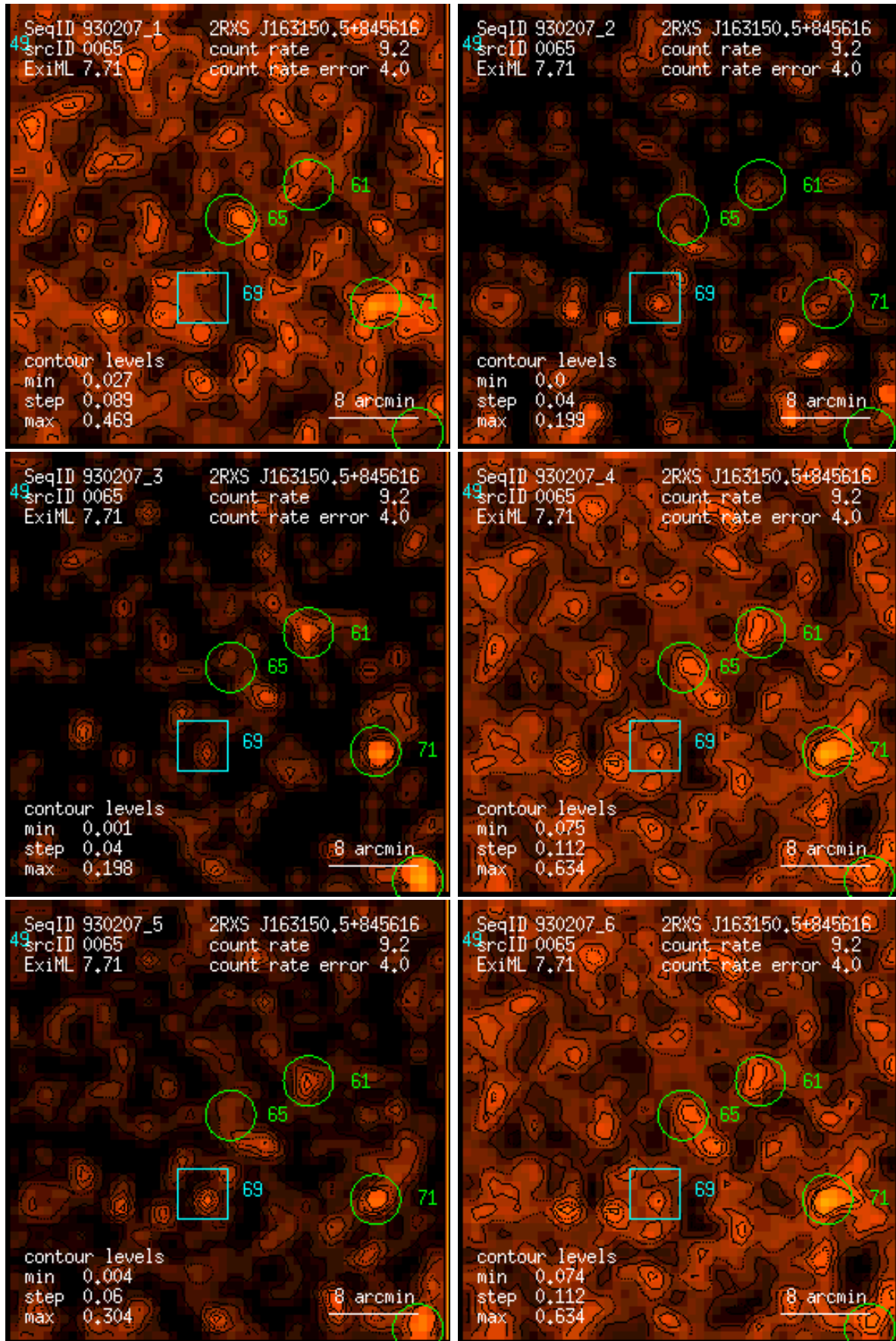
Figure 65: RASS 930207: detection 0065: band rate images, Gaussian filter: (1) PSPC channels 11 – 41, (2) 52 – 90, (3) 91 – 201, (4) 11 – 235, (5) 52 – 201, (6) 11 – 201. Broad band rates in counts/ks. Band rate contour levels in counts/ks/arcmin 2 .
