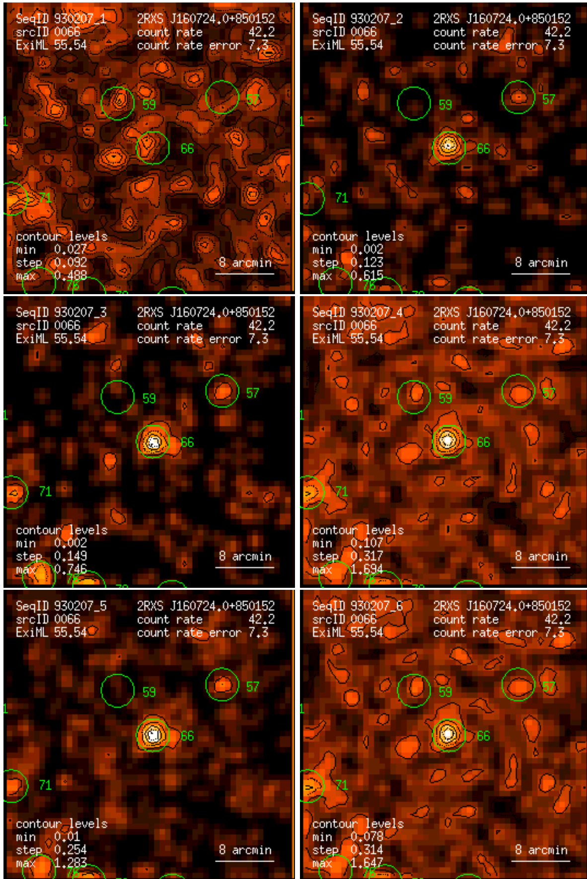
Figure 66: RASS 930207: detection 0066: band rate images, Gaussian filter: (1) PSPC channels 11 – 41, (2) 52 – 90, (3) 91 – 201, (4) 11 – 235, (5) 52 – 201, (6) 11 – 201. Broad band rates in counts/ks. Band rate contour levels in counts/ks/arcmin 2 .
