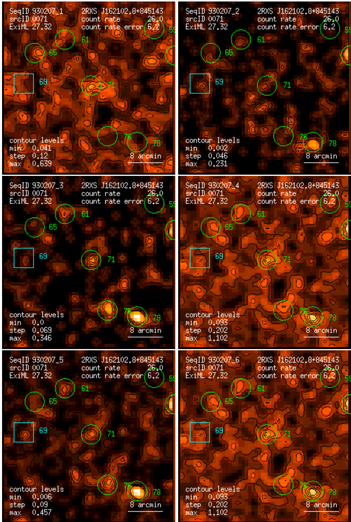
Figure 71: RASS 930207: detection 0071: band rate images, Gaussian filter: (1) PSPC channels 11 – 41, (2) 52 – 90, (3) 91 – 201, (4) 11 – 235, (5) 52 – 201, (6) 11 – 201. Broad band rates in counts/ks. Band rate contour levels in counts/ks/arcmin 2 .
