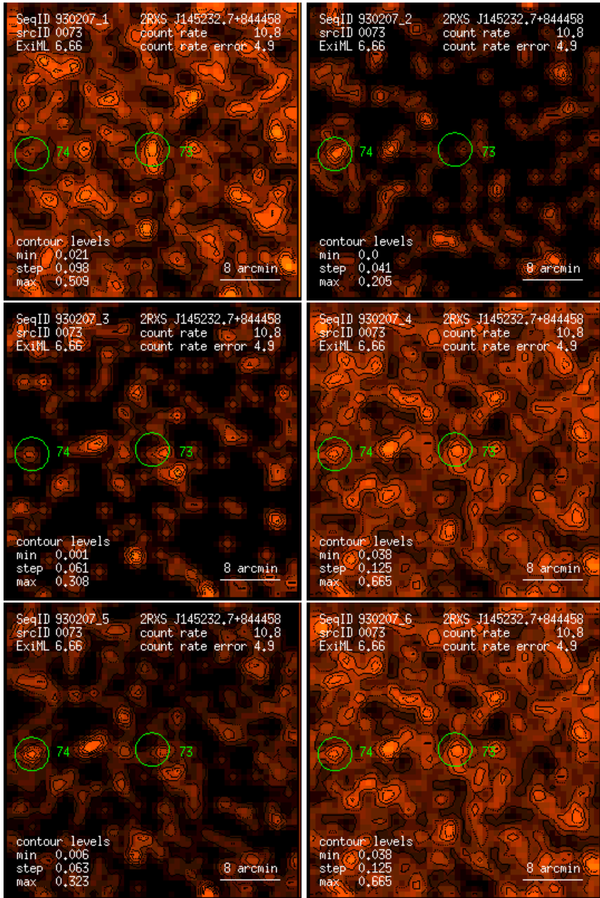
Figure 73: RASS 930207: detection 0073: band rate images, Gaussian filter: (1) PSPC channels 11 – 41, (2) 52 – 90, (3) 91 – 201, (4) 11 – 235, (5) 52 – 201, (6) 11 – 201. Broad band rates in counts/ks. Band rate contour levels in counts/ks/arcmin 2 .
