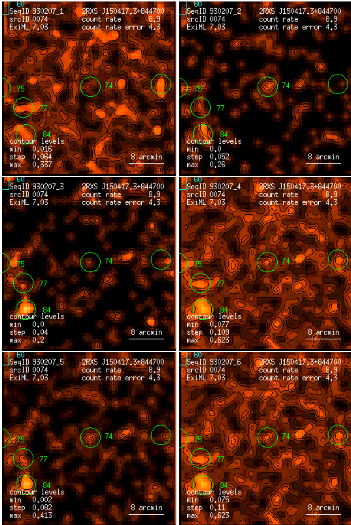
Figure 74: RASS 930207: detection 0074: band rate images, Gaussian filter: (1) PSPC channels 11 – 41, (2) 52 – 90, (3) 91 – 201, (4) 11 – 235, (5) 52 – 201, (6) 11 – 201. Broad band rates in counts/ks. Band rate contour levels in counts/ks/arcmin 2 .
