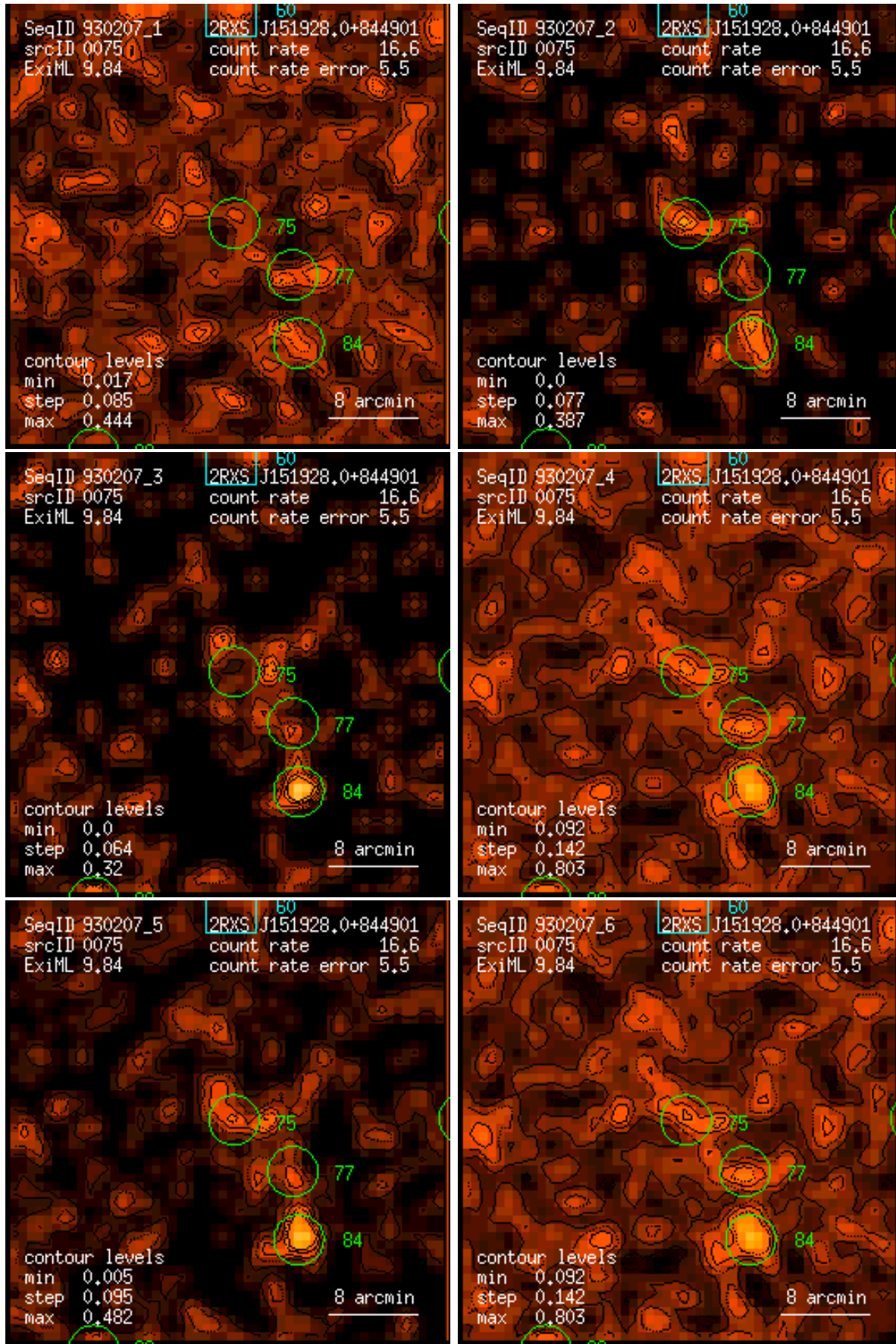
Figure 75: RASS 930207: detection 0075: band rate images, Gaussian filter: (1) PSPC channels 11 – 41, (2) 52 – 90, (3) 91 – 201, (4) 11 – 235, (5) 52 – 201, (6) 11 – 201. Broad band rates in counts/ks. Band rate contour levels in counts/ks/arcmin 2 .
