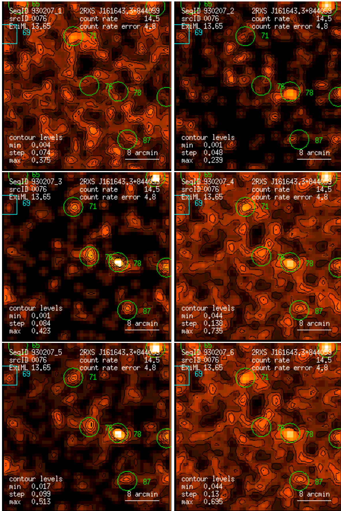
Figure 76: RASS 930207: detection 0076: band rate images, Gaussian filter: (1) PSPC channels 11 – 41, (2) 52 – 90, (3) 91 – 201, (4) 11 – 235, (5) 52 – 201, (6) 11 – 201. Broad band rates in counts/ks. Band rate contour levels in counts/ks/arcmin 2 .
