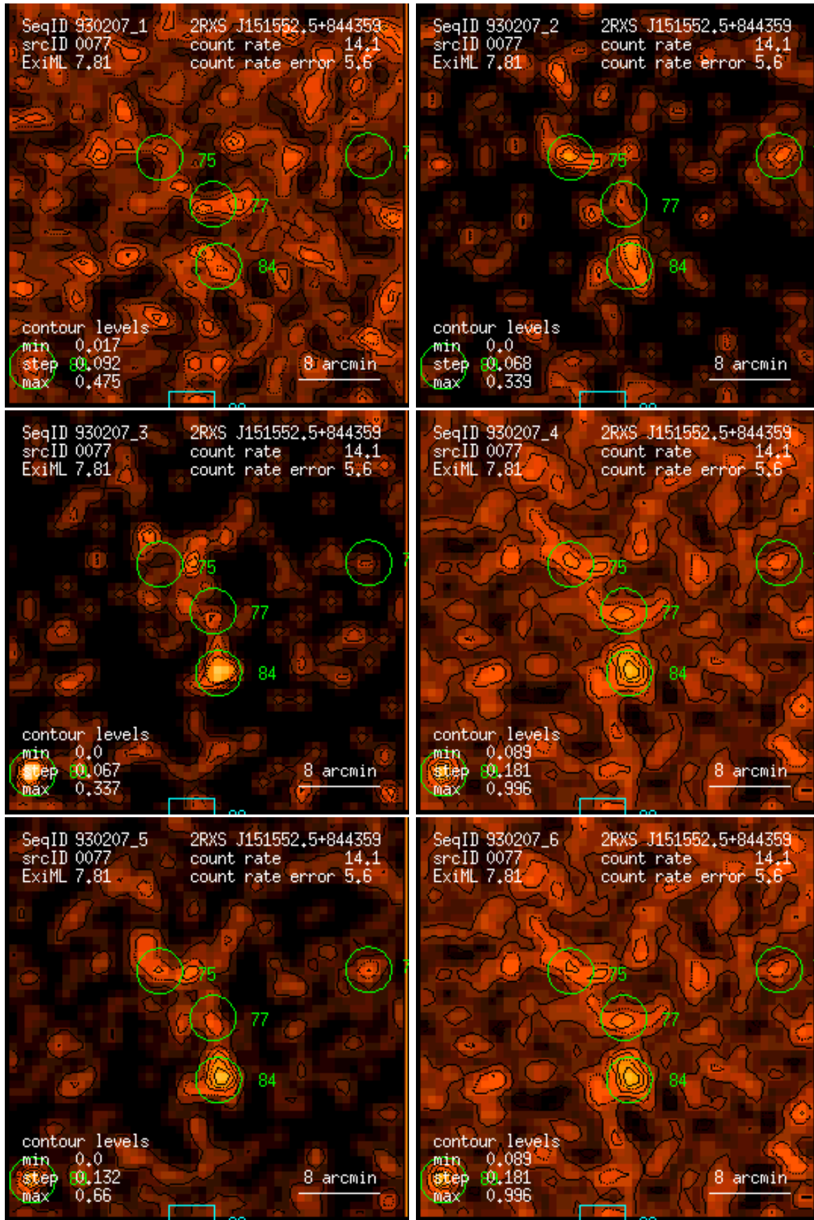
Figure 77: RASS 930207: detection 0077: band rate images, Gaussian filter: (1) PSPC channels 11 – 41, (2) 52 – 90, (3) 91 – 201, (4) 11 – 235, (5) 52 – 201, (6) 11 – 201. Broad band rates in counts/ks. Band rate contour levels in counts/ks/arcmin 2 .
