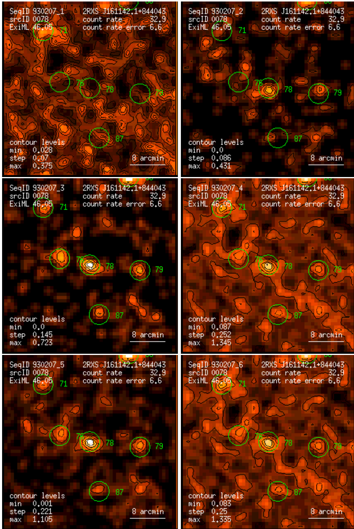
Figure 78: RASS 930207: detection 0078: band rate images, Gaussian filter: (1) PSPC channels 11 – 41, (2) 52 – 90, (3) 91 – 201, (4) 11 – 235, (5) 52 – 201, (6) 11 – 201. Broad band rates in counts/ks. Band rate contour levels in counts/ks/arcmin 2 .
