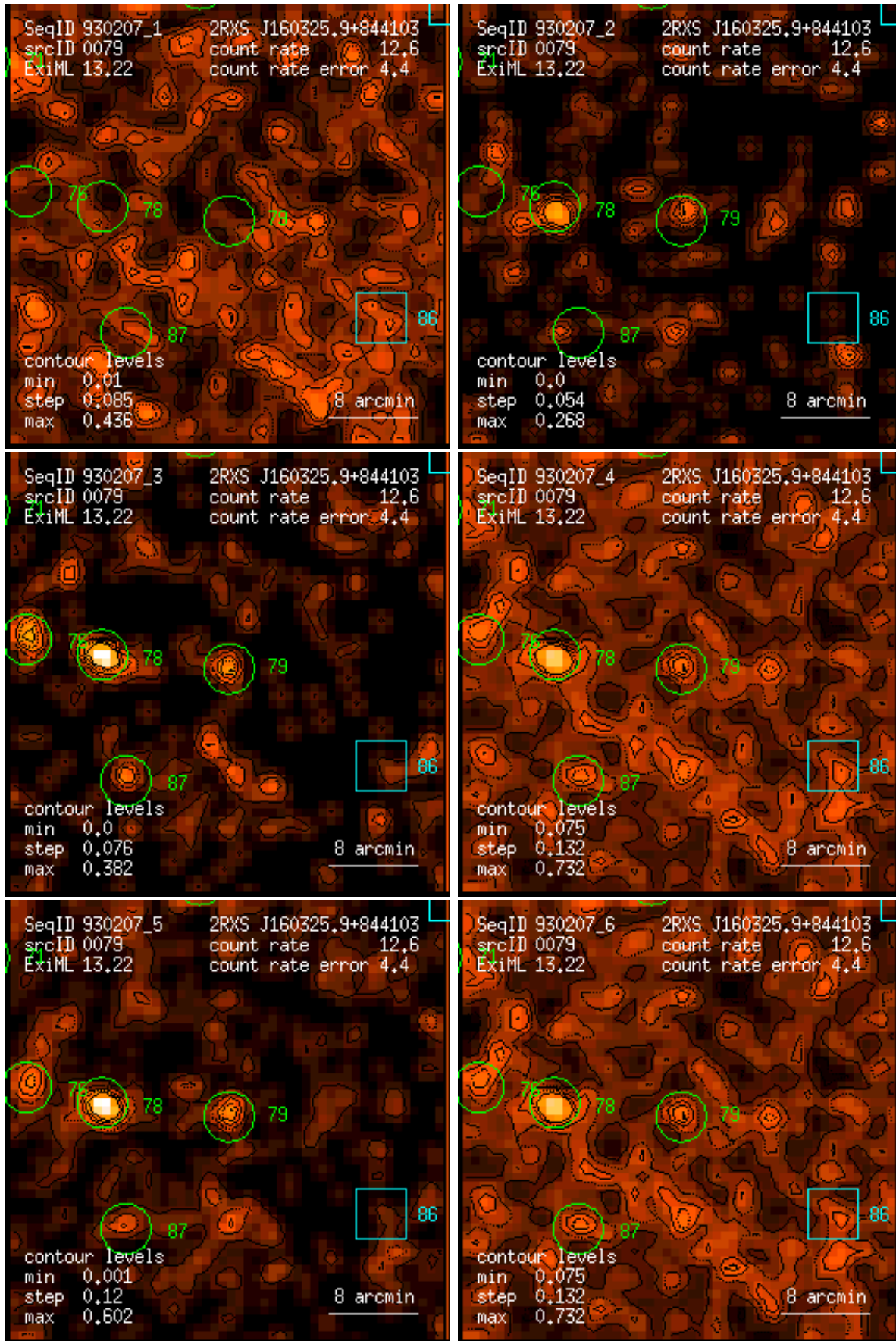
Figure 79: RASS 930207: detection 0079: band rate images, Gaussian filter: (1) PSPC channels 11 – 41, (2) 52 – 90, (3) 91 – 201, (4) 11 – 235, (5) 52 – 201, (6) 11 – 201. Broad band rates in counts/ks. Band rate contour levels in counts/ks/arcmin 2 .
