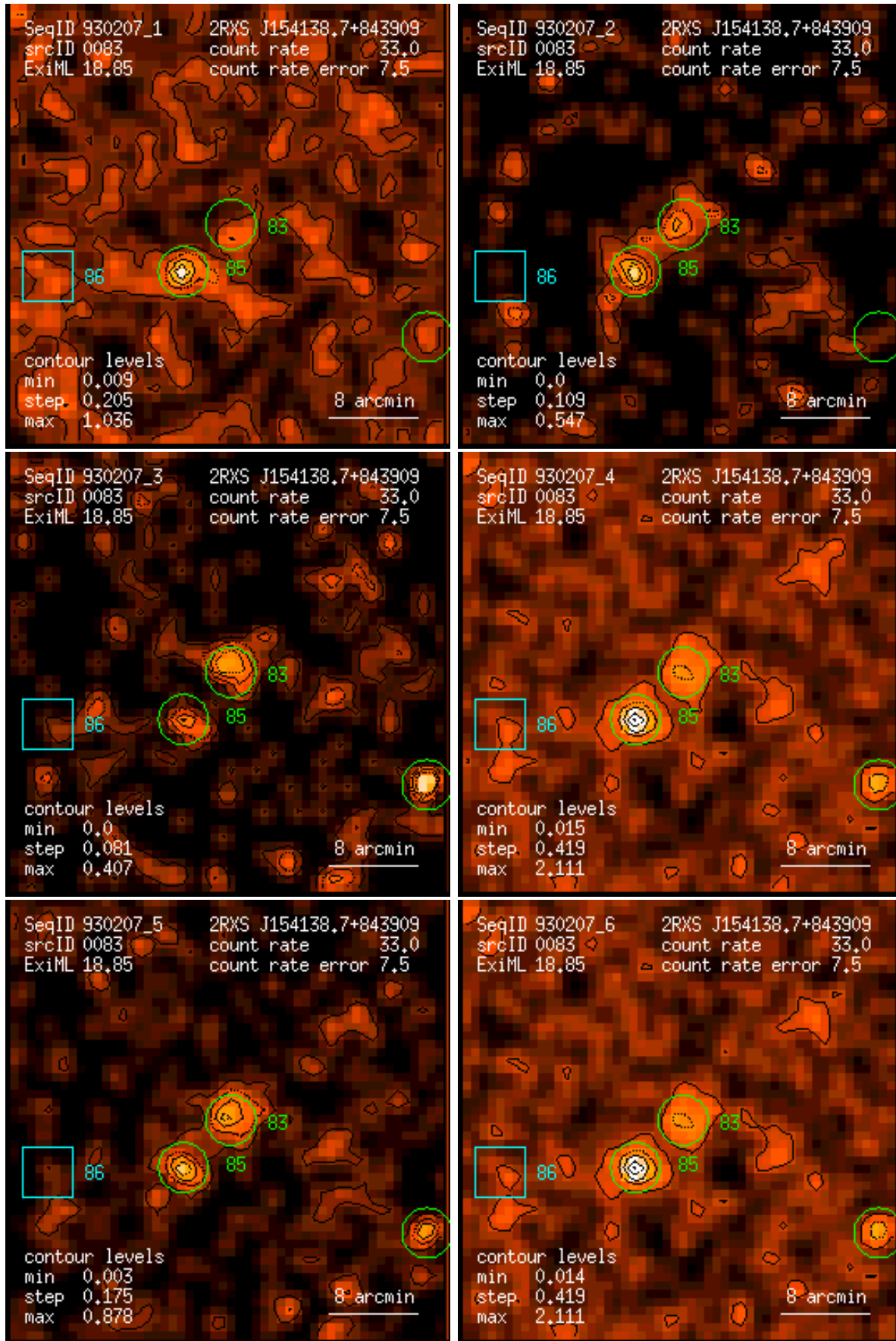
Figure 83: RASS 930207: detection 0083: band rate images, Gaussian filter: (1) PSPC channels 11 – 41, (2) 52 – 90, (3) 91 – 201, (4) 11 – 235, (5) 52 – 201, (6) 11 – 201. Broad band rates in counts/ks. Band rate contour levels in counts/ks/arcmin 2 .
