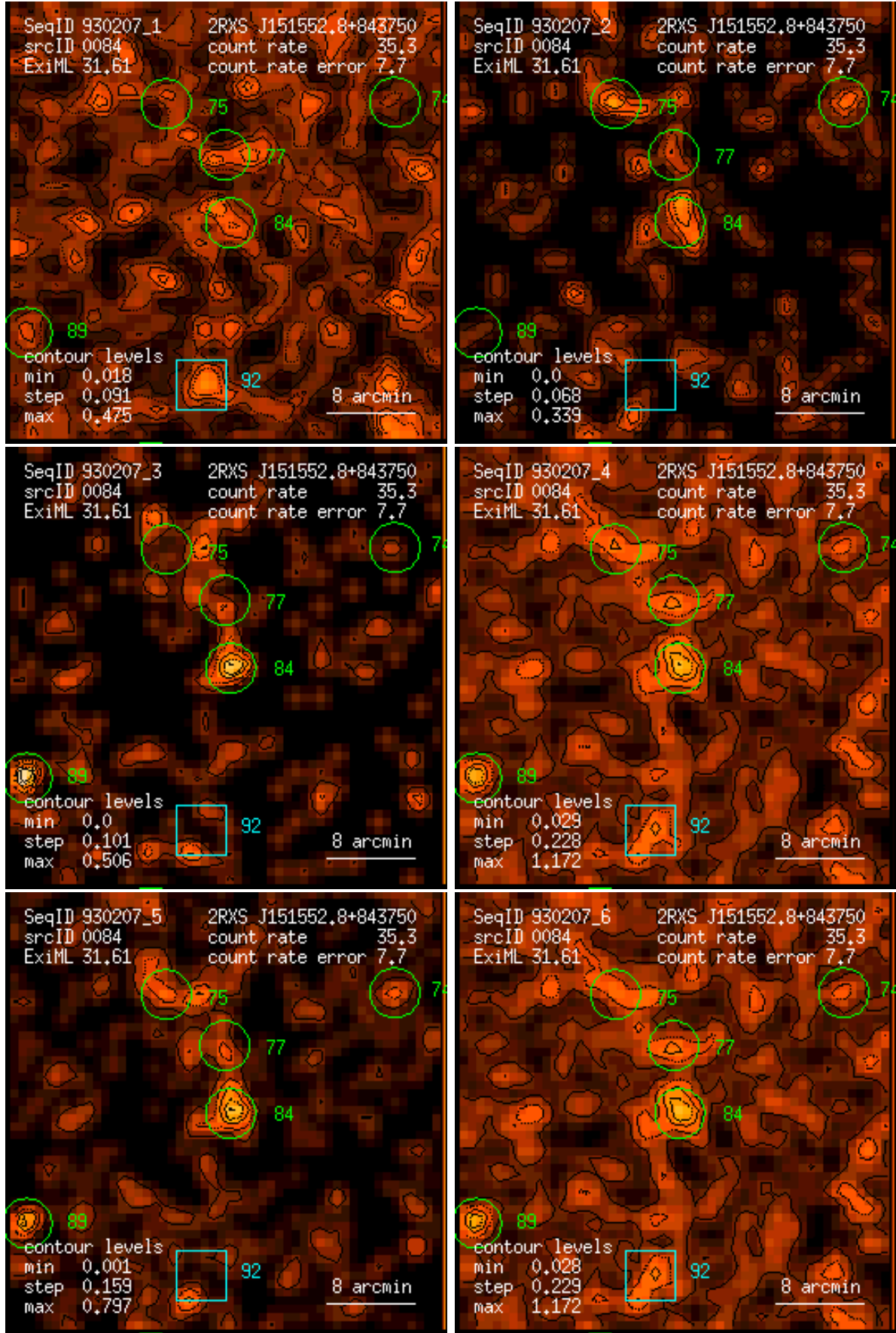
Figure 84: RASS 930207: detection 0084: band rate images, Gaussian filter: (1) PSPC channels 11 – 41, (2) 52 – 90, (3) 91 – 201, (4) 11 – 235, (5) 52 – 201, (6) 11 – 201. Broad band rates in counts/ks. Band rate contour levels in counts/ks/arcmin 2 .
