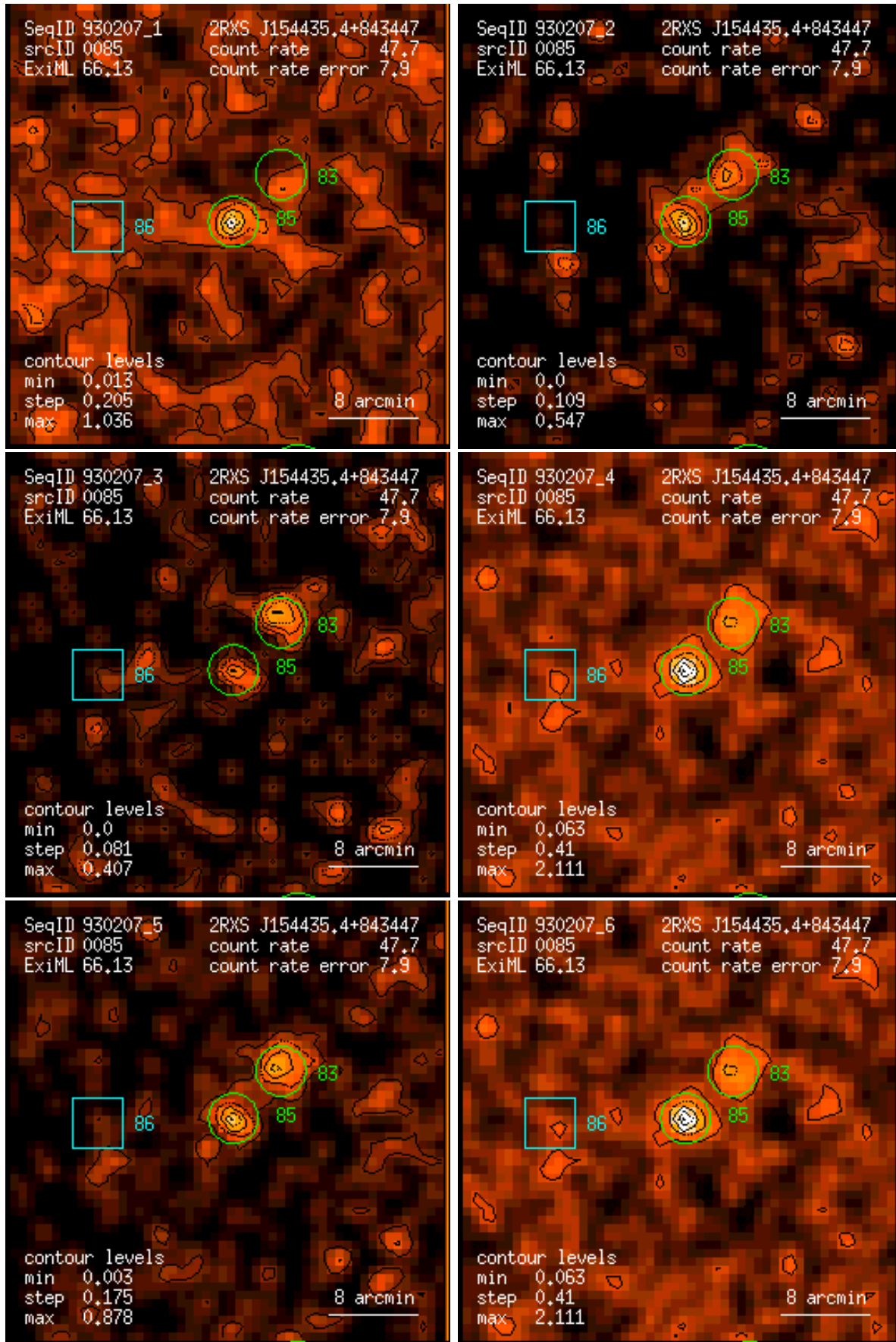
Figure 85: RASS 930207: detection 0085: band rate images, Gaussian filter: (1) PSPC channels 11 – 41, (2) 52 – 90, (3) 91 – 201, (4) 11 – 235, (5) 52 – 201, (6) 11 – 201. Broad band rates in counts/ks. Band rate contour levels in counts/ks/arcmin 2 .
