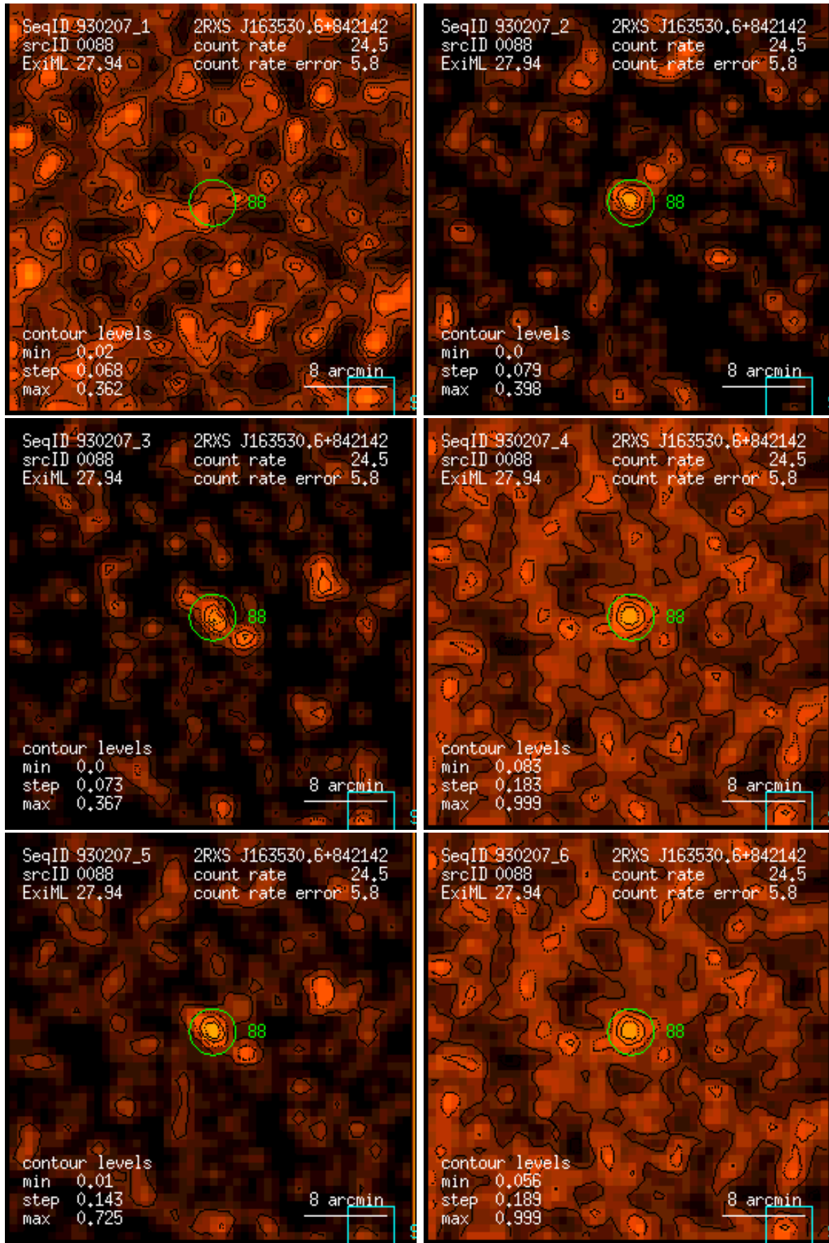
Figure 88: RASS 930207: detection 0088: band rate images, Gaussian filter: (1) PSPC channels 11 – 41, (2) 52 – 90, (3) 91 – 201, (4) 11 – 235, (5) 52 – 201, (6) 11 – 201. Broad band rates in counts/ks. Band rate contour levels in counts/ks/arcmin 2 .
