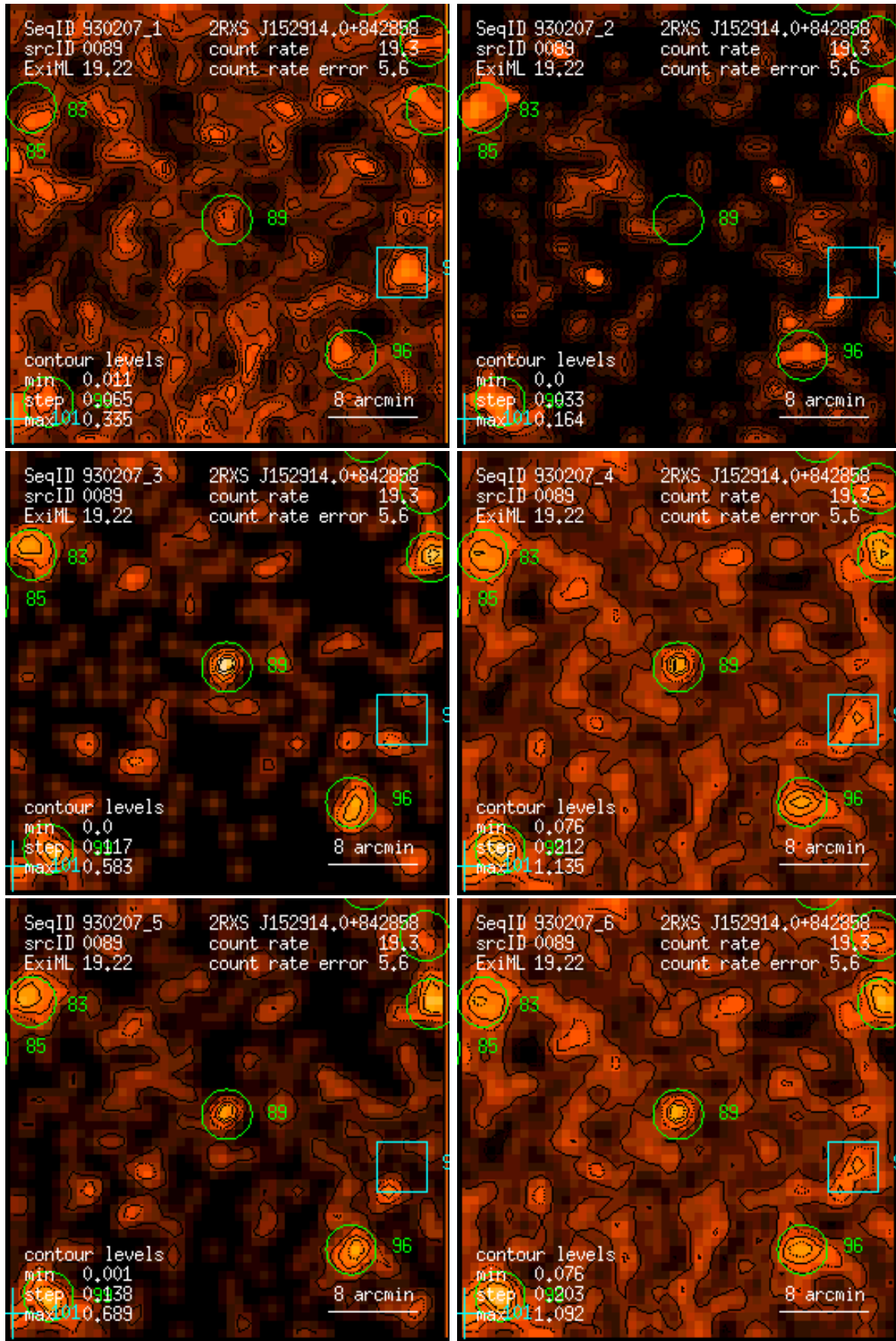
Figure 89: RASS 930207: detection 0089: band rate images, Gaussian filter: (1) PSPC channels 11 – 41, (2) 52 – 90, (3) 91 – 201, (4) 11 – 235, (5) 52 – 201, (6) 11 – 201. Broad band rates in counts/ks. Band rate contour levels in counts/ks/arcmin 2 .
