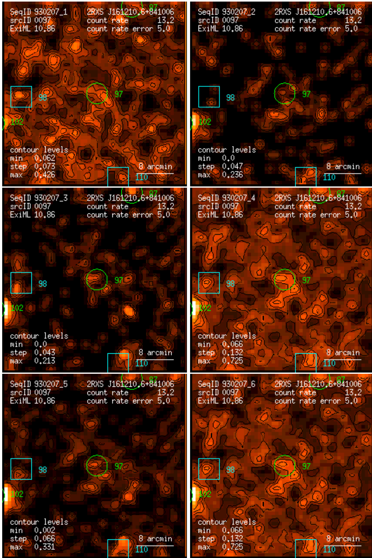
Figure 97: RASS 930207: detection 0097: band rate images, Gaussian filter: (1) PSPC channels 11 – 41, (2) 52 – 90, (3) 91 – 201, (4) 11 – 235, (5) 52 – 201, (6) 11 – 201. Broad band rates in counts/ks. Band rate contour levels in counts/ks/arcmin 2 .
