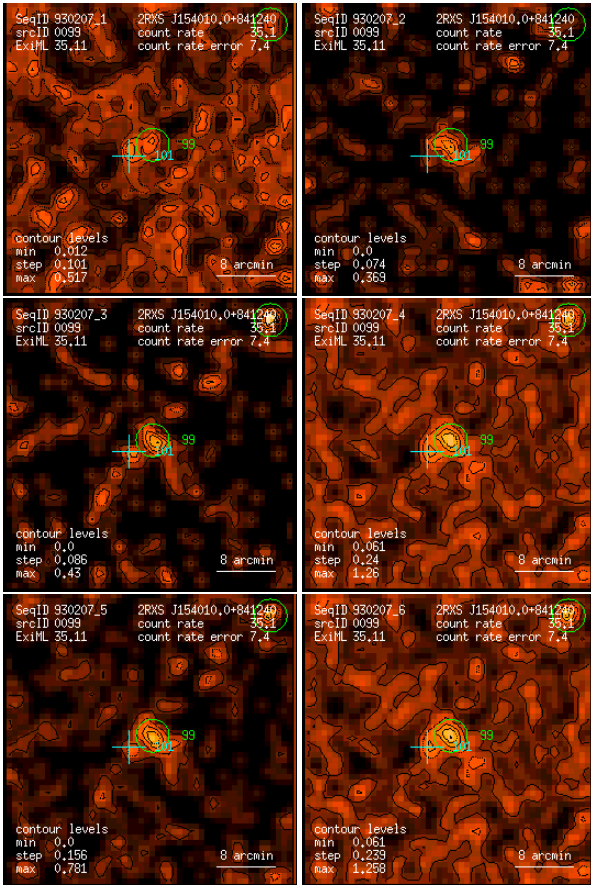
Figure 99: RASS 930207: detection 0099: band rate images, Gaussian filter: (1) PSPC channels 11 – 41, (2) 52 – 90, (3) 91 – 201, (4) 11 – 235, (5) 52 – 201, (6) 11 – 201. Broad band rates in counts/ks. Band rate contour levels in counts/ks/arcmin 2 .
