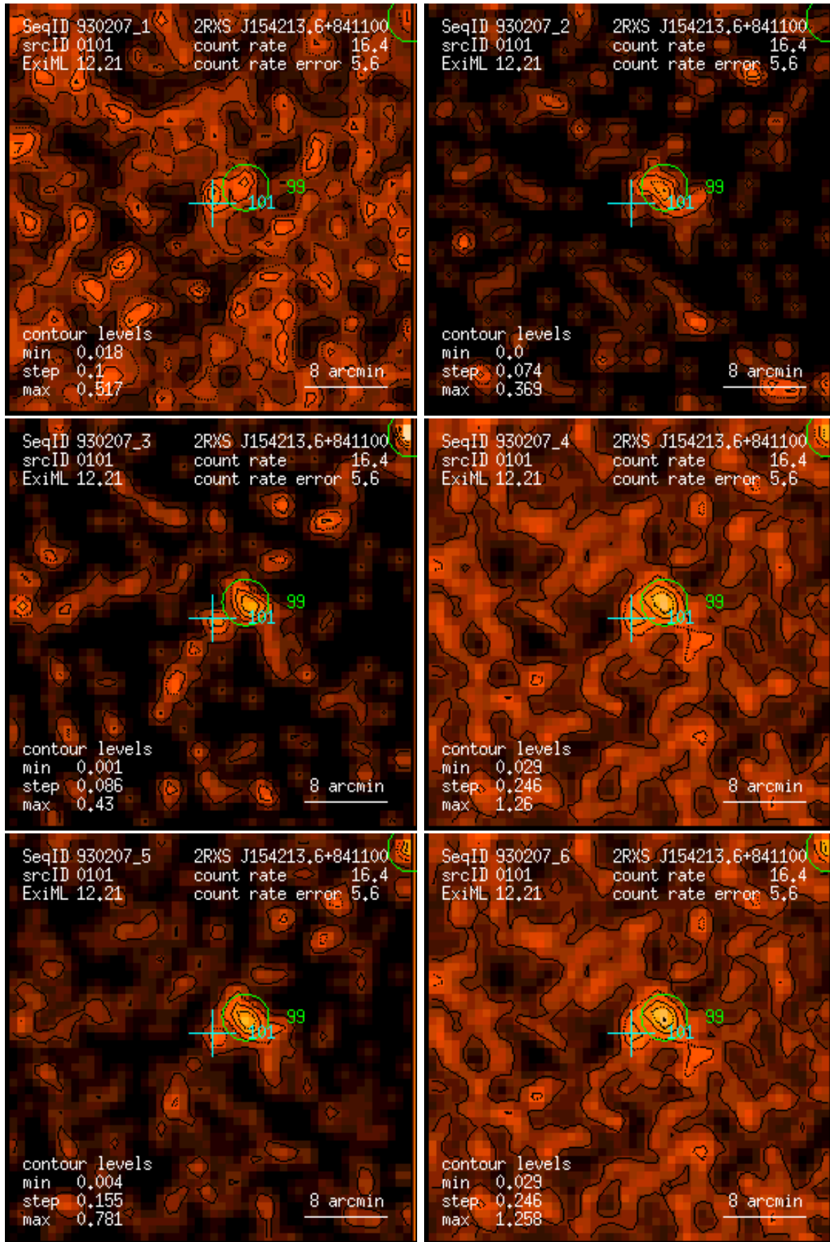
Figure 101: RASS 930207: detection 0101: band rate images, Gaussian filter: (1) PSPC channels 11 – 41, (2) 52 – 90, (3) 91 – 201, (4) 11 – 235, (5) 52 – 201, (6) 11 – 201. Broad band rates in counts/ks. Band rate contour levels in counts/ks/arcmin 2 .
