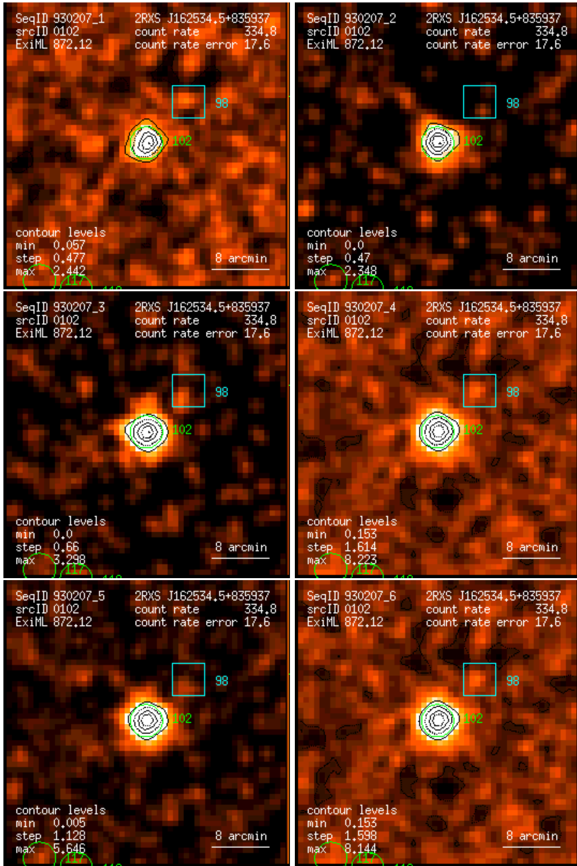
Figure 102: RASS 930207: detection 0102: band rate images, Gaussian filter: (1) PSPC channels 11 – 41, (2) 52 – 90, (3) 91 – 201, (4) 11 – 235, (5) 52 – 201, (6) 11 – 201. Broad band rates in counts/ks. Band rate contour levels in counts/ks/arcmin 2 .
