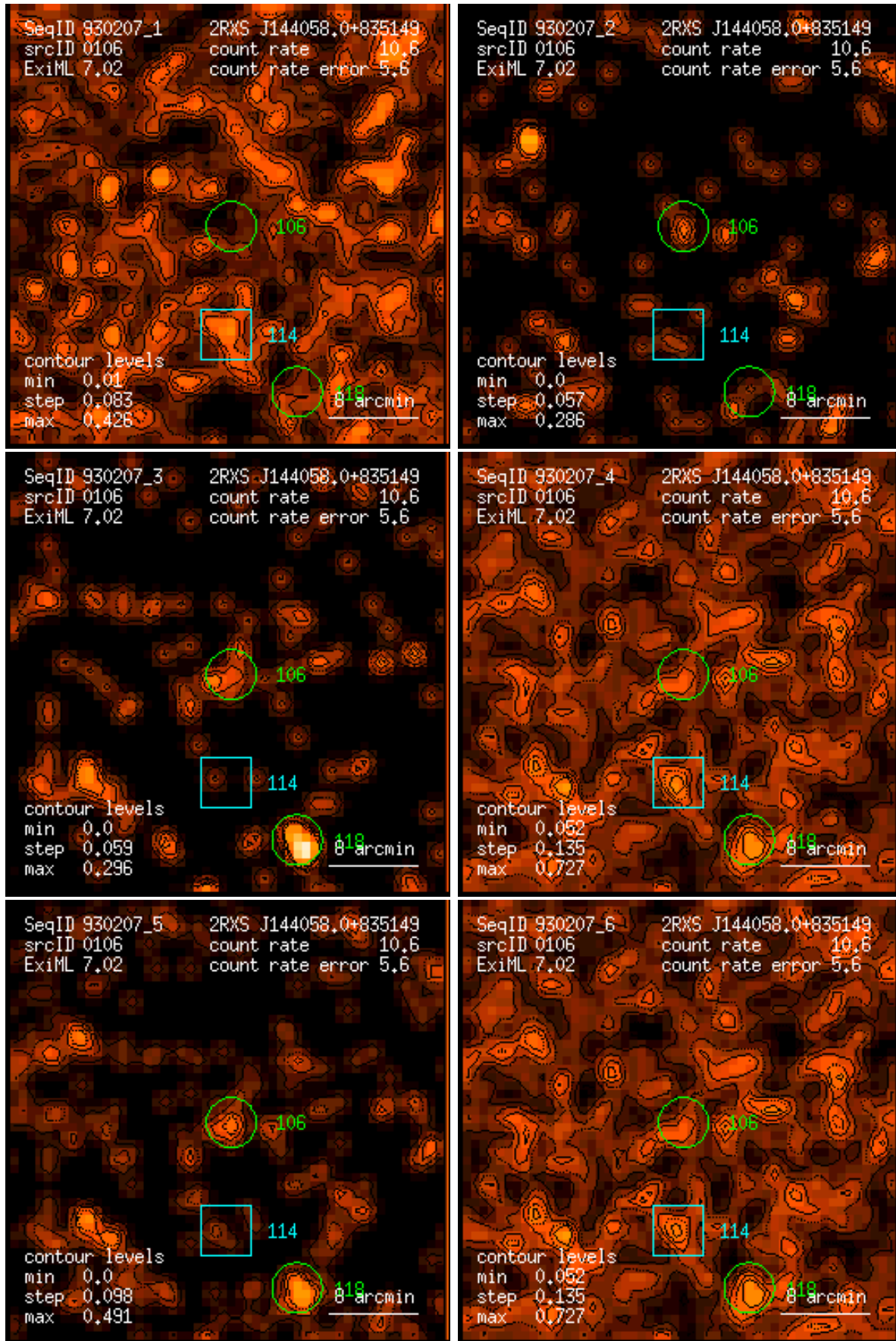
Figure 106: RASS 930207: detection 0106: band rate images, Gaussian filter: (1) PSPC channels 11 – 41, (2) 52 – 90, (3) 91 – 201, (4) 11 – 235, (5) 52 – 201, (6) 11 – 201. Broad band rates in counts/ks. Band rate contour levels in counts/ks/arcmin 2 .
