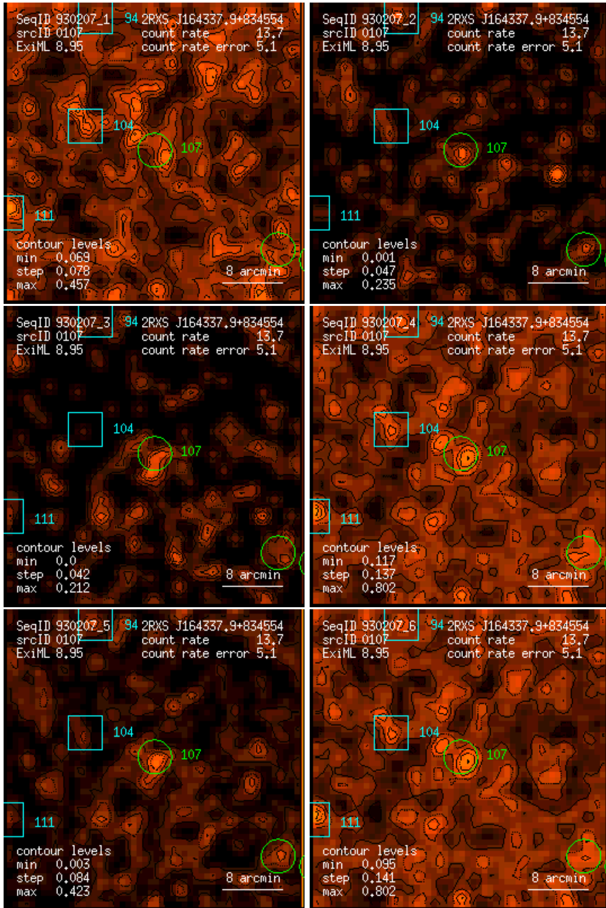
Figure 107: RASS 930207: detection 0107: band rate images, Gaussian filter: (1) PSPC channels 11 – 41, (2) 52 – 90, (3) 91 – 201, (4) 11 – 235, (5) 52 – 201, (6) 11 – 201. Broad band rates in counts/ks. Band rate contour levels in counts/ks/arcmin 2 .
