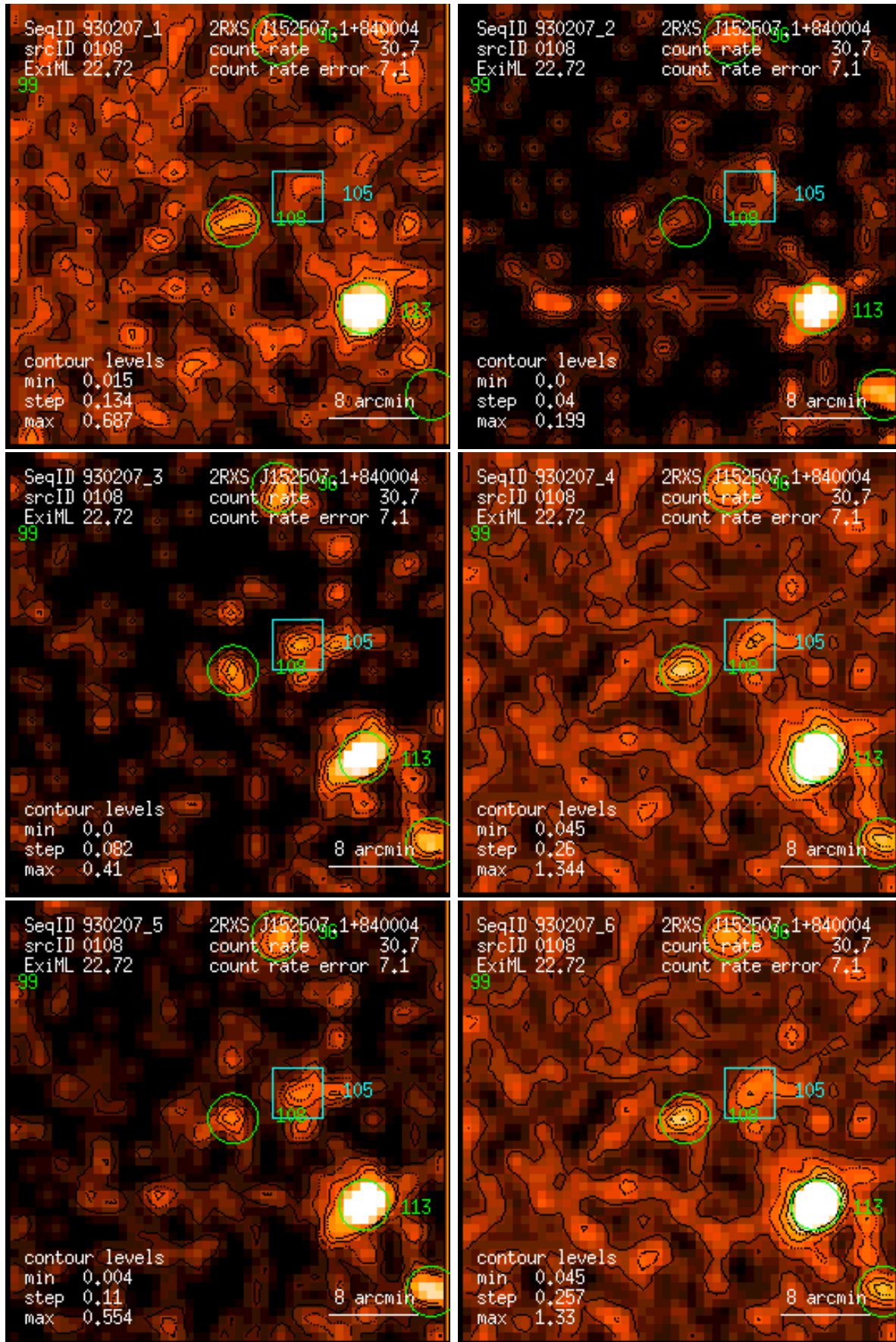
Figure 108: RASS 930207: detection 0108: band rate images, Gaussian filter: (1) PSPC channels 11 – 41, (2) 52 – 90, (3) 91 – 201, (4) 11 – 235, (5) 52 – 201, (6) 11 – 201. Broad band rates in counts/ks. Band rate contour levels in counts/ks/arcmin 2 .
