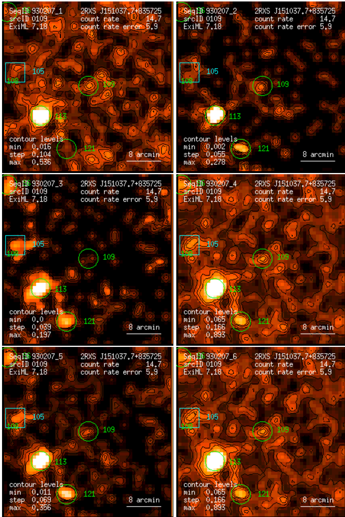
Figure 109: RASS 930207: detection 0109: band rate images, Gaussian filter: (1) PSPC channels 11 – 41, (2) 52 – 90, (3) 91 – 201, (4) 11 – 235, (5) 52 – 201, (6) 11 – 201. Broad band rates in counts/ks. Band rate contour levels in counts/ks/arcmin 2 .
