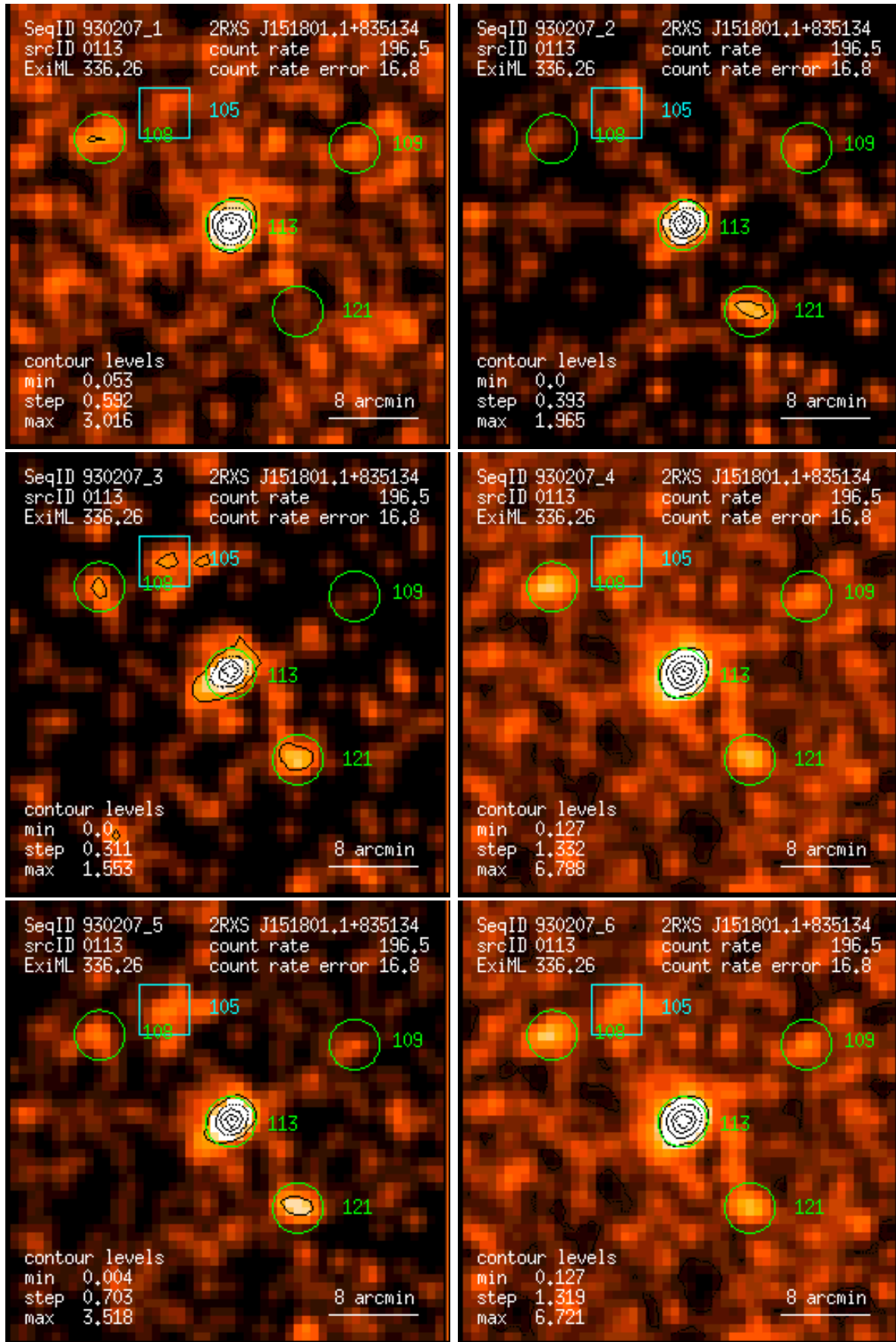
Figure 113: RASS 930207: detection 0113: band rate images, Gaussian filter: (1) PSPC channels 11 – 41, (2) 52 – 90, (3) 91 – 201, (4) 11 – 235, (5) 52 – 201, (6) 11 – 201. Broad band rates in counts/ks. Band rate contour levels in counts/ks/arcmin 2 .
