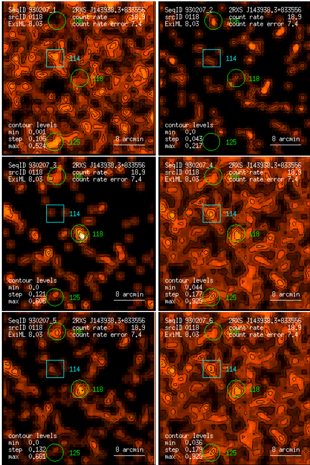
Figure 118: RASS 930207: detection 0118: band rate images, Gaussian filter: (1) PSPC channels 11 – 41, (2) 52 – 90, (3) 91 – 201, (4) 11 – 235, (5) 52 – 201, (6) 11 – 201. Broad band rates in counts/ks. Band rate contour levels in counts/ks/arcmin 2 .
