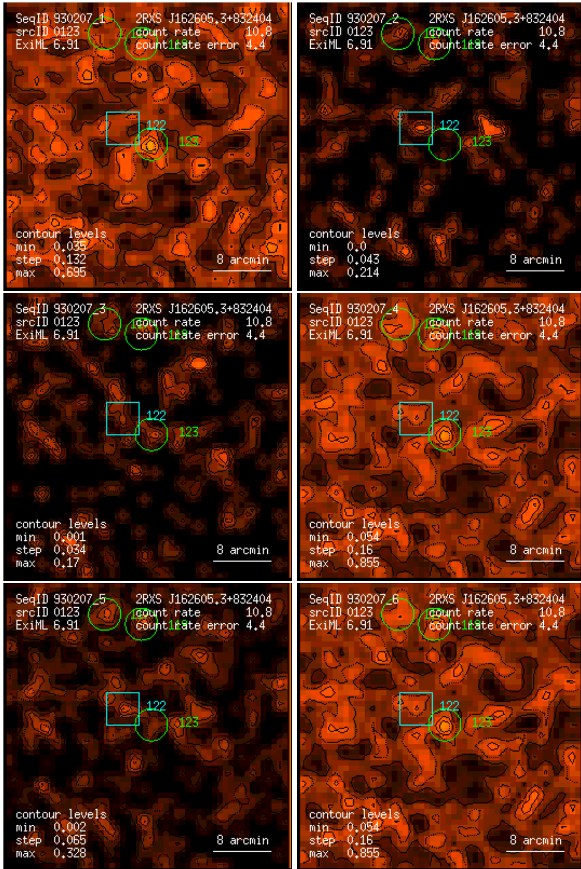
Figure 123: RASS 930207: detection 0123: band rate images, Gaussian filter: (1) PSPC channels 11 – 41, (2) 52 – 90, (3) 91 – 201, (4) 11 – 235, (5) 52 – 201, (6) 11 – 201. Broad band rates in counts/ks. Band rate contour levels in counts/ks/arcmin 2 .
