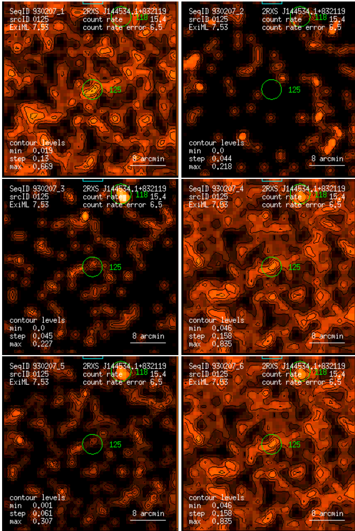
Figure 125: RASS 930207: detection 0125: band rate images, Gaussian filter: (1) PSPC channels 11 – 41, (2) 52 – 90, (3) 91 – 201, (4) 11 – 235, (5) 52 – 201, (6) 11 – 201. Broad band rates in counts/ks. Band rate contour levels in counts/ks/arcmin 2 .
