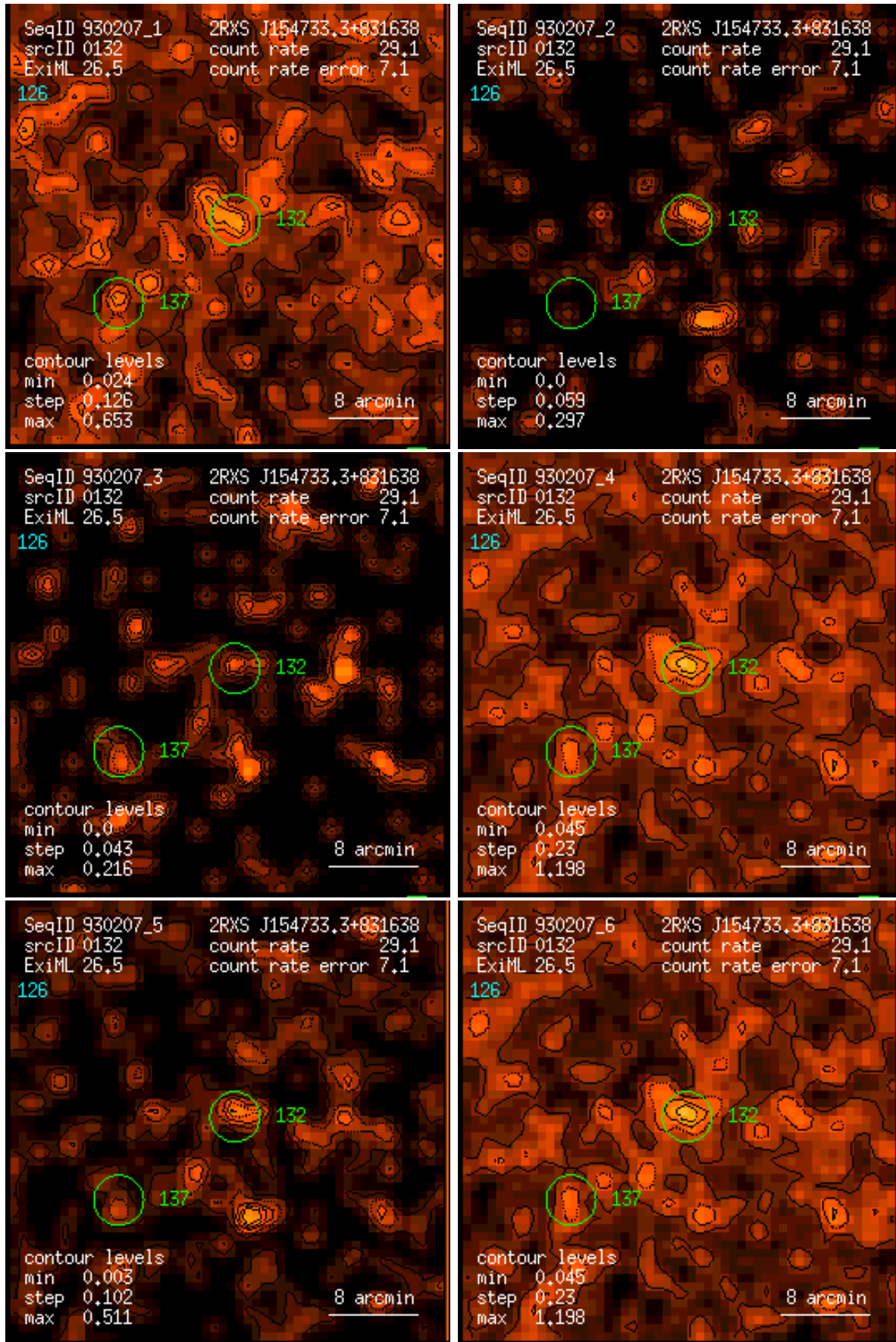
Figure 132: RASS 930207: detection 0132: band rate images, Gaussian filter: (1) PSPC channels 11 – 41, (2) 52 – 90, (3) 91 – 201, (4) 11 – 235, (5) 52 – 201, (6) 11 – 201. Broad band rates in counts/ks. Band rate contour levels in counts/ks/arcmin 2 .
