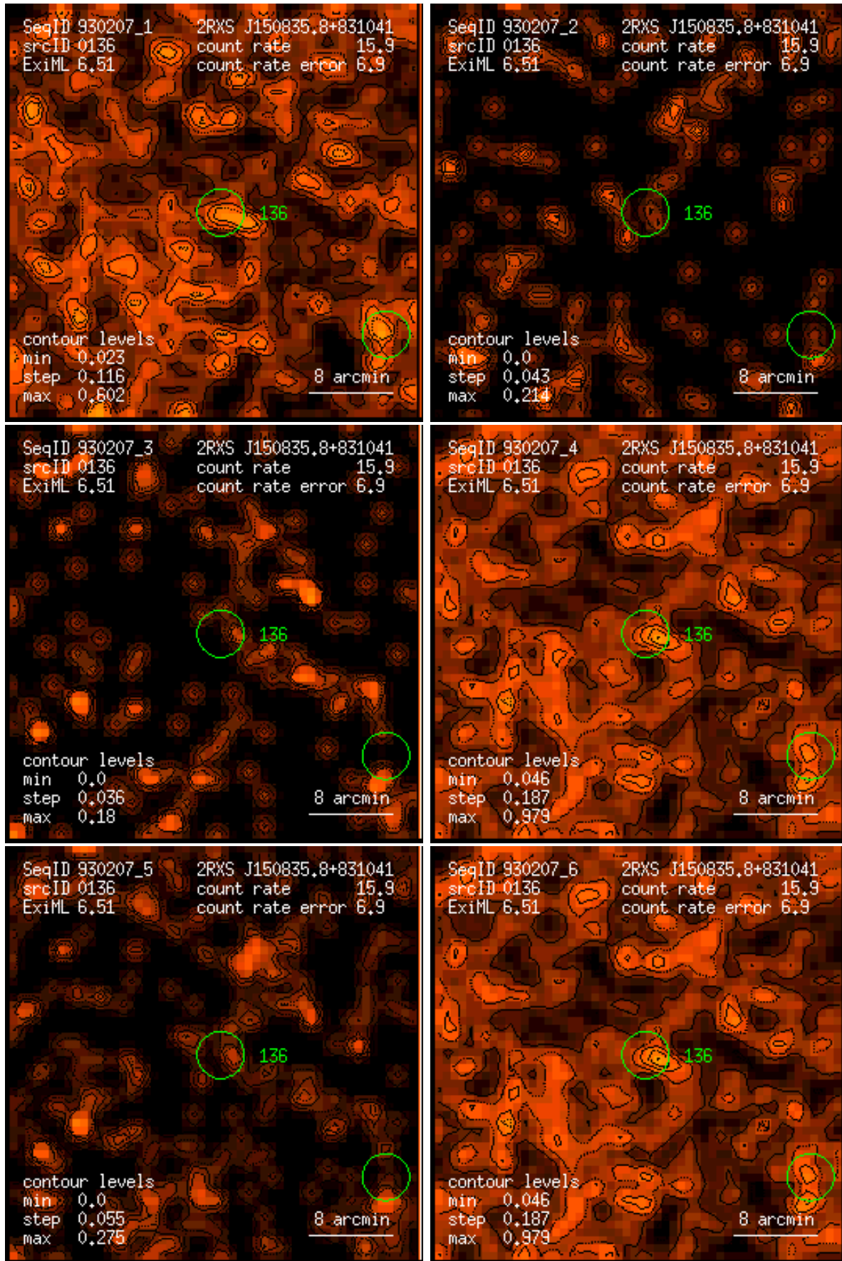
Figure 136: RASS 930207: detection 0136: band rate images, Gaussian filter: (1) PSPC channels 11 – 41, (2) 52 – 90, (3) 91 – 201, (4) 11 – 235, (5) 52 – 201, (6) 11 – 201. Broad band rates in counts/ks. Band rate contour levels in counts/ks/arcmin 2 .
