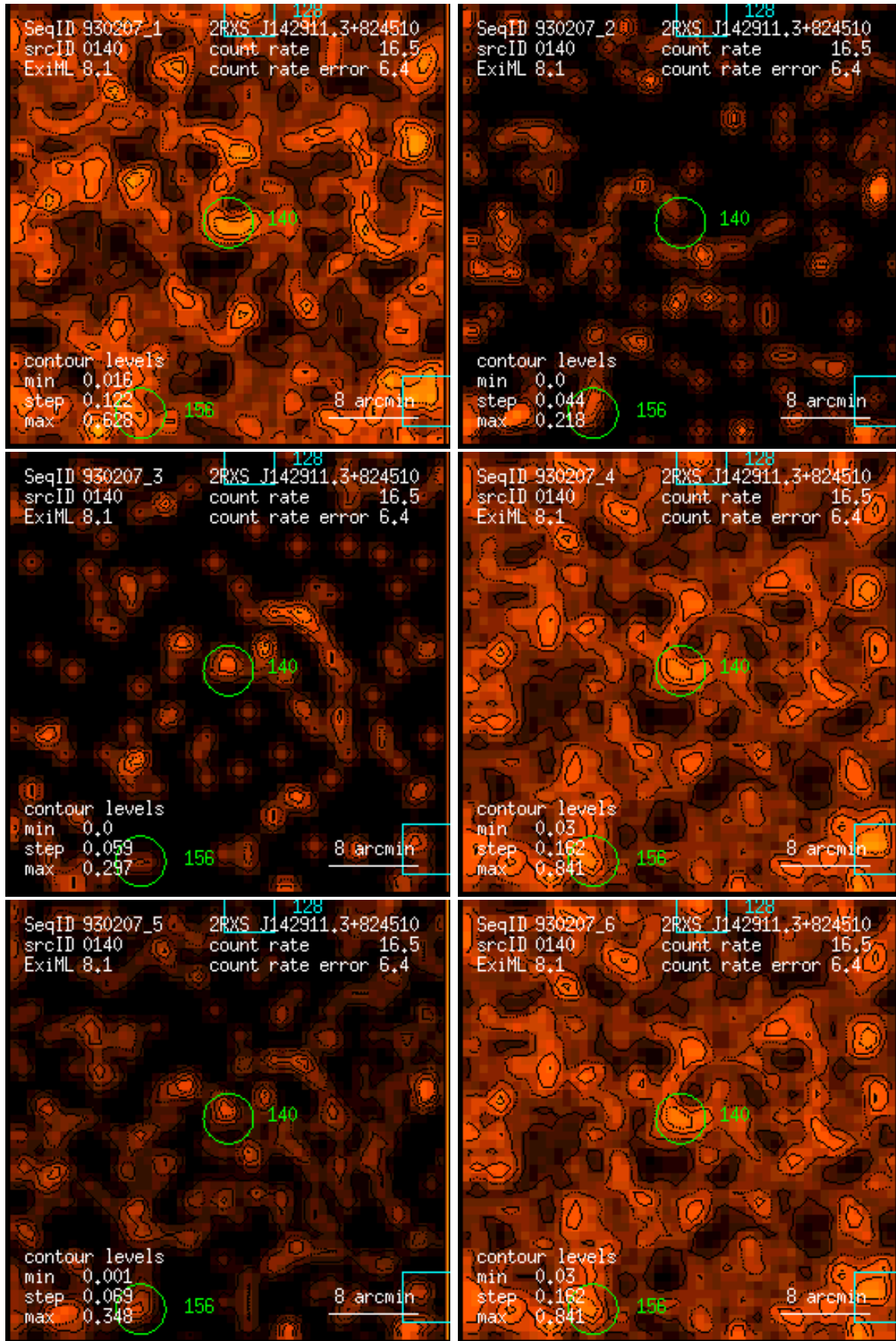
Figure 140: RASS 930207: detection 0140: band rate images, Gaussian filter: (1) PSPC channels 11 – 41, (2) 52 – 90, (3) 91 – 201, (4) 11 – 235, (5) 52 – 201, (6) 11 – 201. Broad band rates in counts/ks. Band rate contour levels in counts/ks/arcmin 2 .
