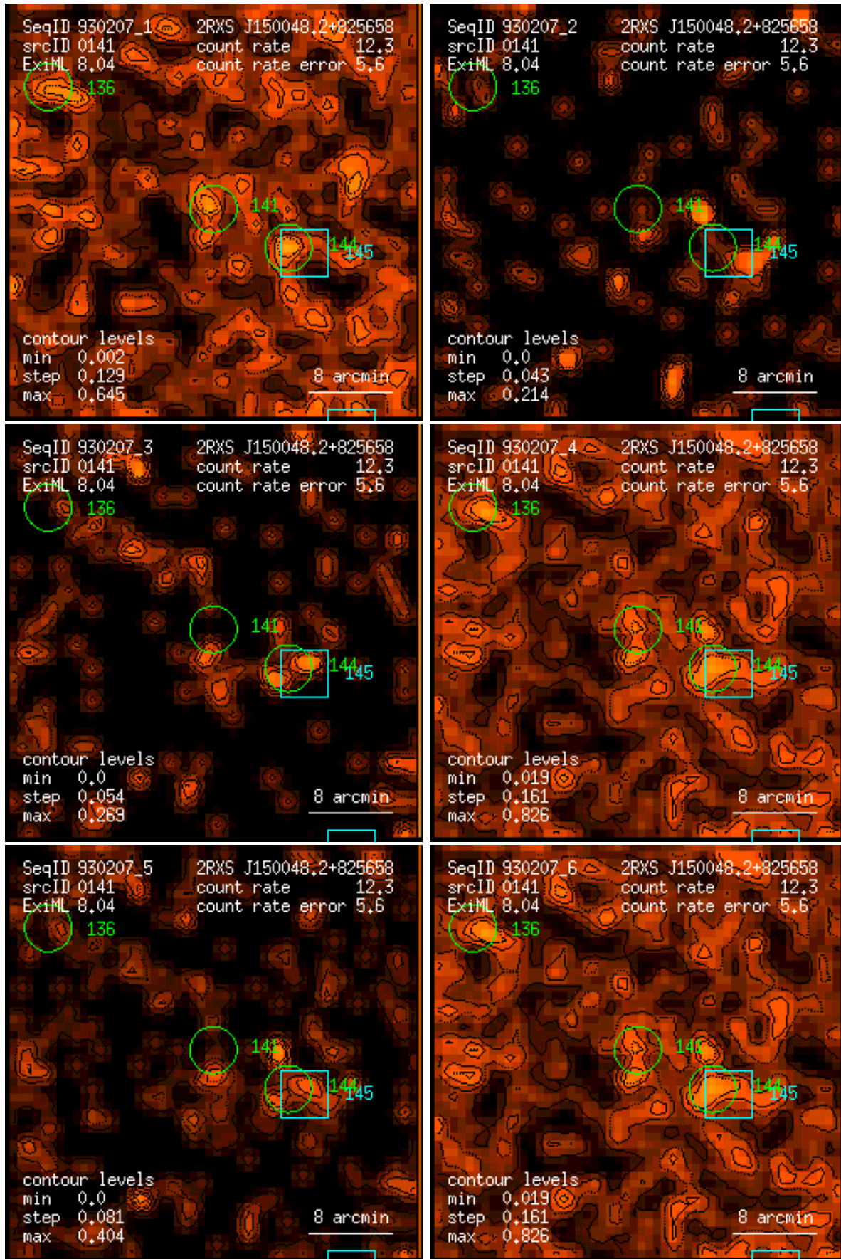
Figure 141: RASS 930207: detection 0141: band rate images, Gaussian filter: (1) PSPC channels 11 – 41, (2) 52 – 90, (3) 91 – 201, (4) 11 – 235, (5) 52 – 201, (6) 11 – 201. Broad band rates in counts/ks. Band rate contour levels in counts/ks/arcmin 2 .
