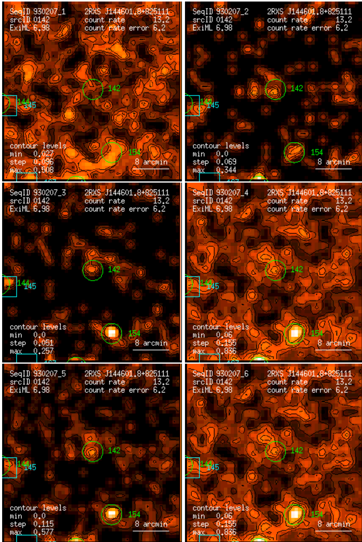
Figure 142: RASS 930207: detection 0142: band rate images, Gaussian filter: (1) PSPC channels 11 – 41, (2) 52 – 90, (3) 91 – 201, (4) 11 – 235, (5) 52 – 201, (6) 11 – 201. Broad band rates in counts/ks. Band rate contour levels in counts/ks/arcmin 2 .
