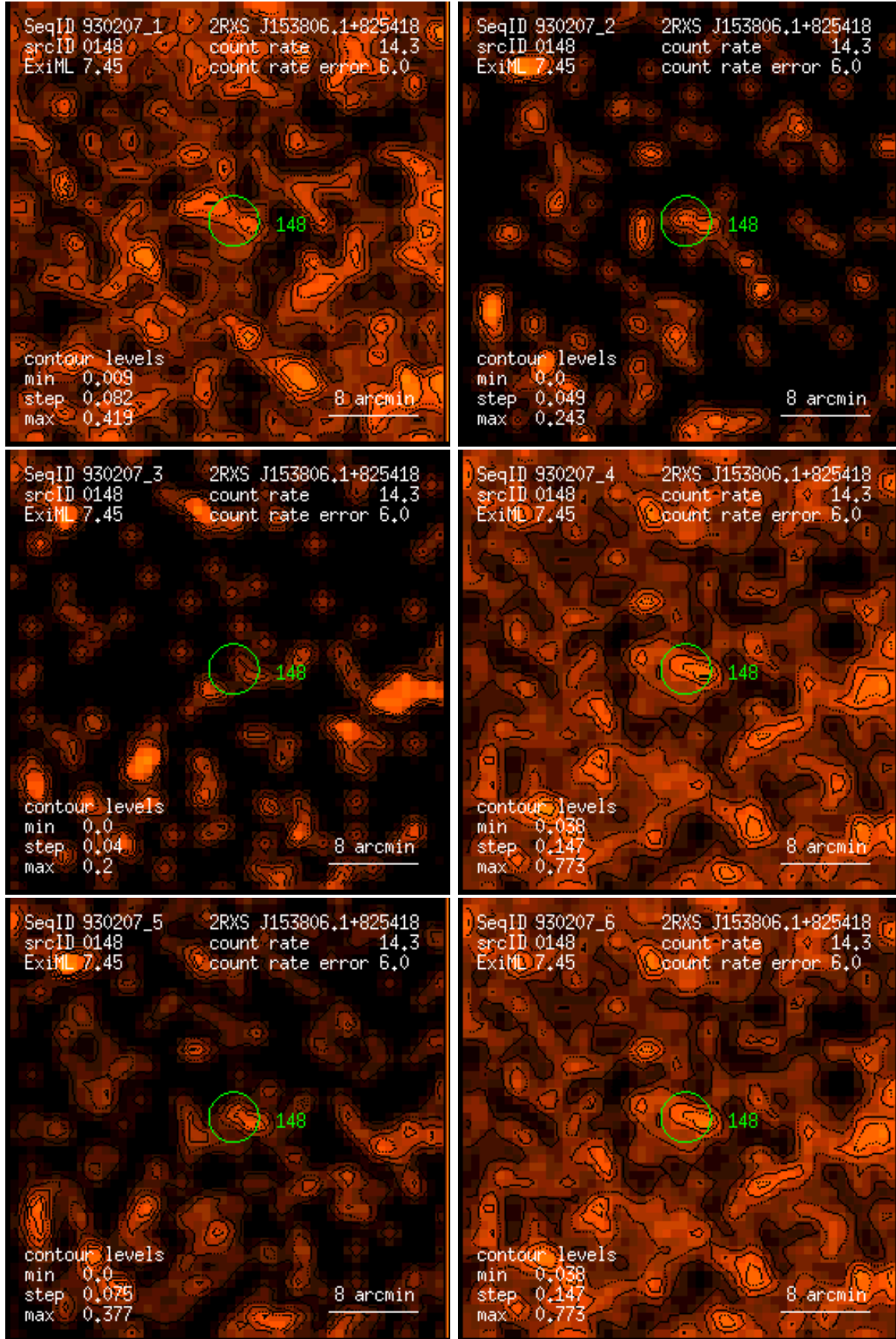
Figure 148: RASS 930207: detection 0148: band rate images, Gaussian filter: (1) PSPC channels 11 – 41, (2) 52 – 90, (3) 91 – 201, (4) 11 – 235, (5) 52 – 201, (6) 11 – 201. Broad band rates in counts/ks. Band rate contour levels in counts/ks/arcmin 2 .
