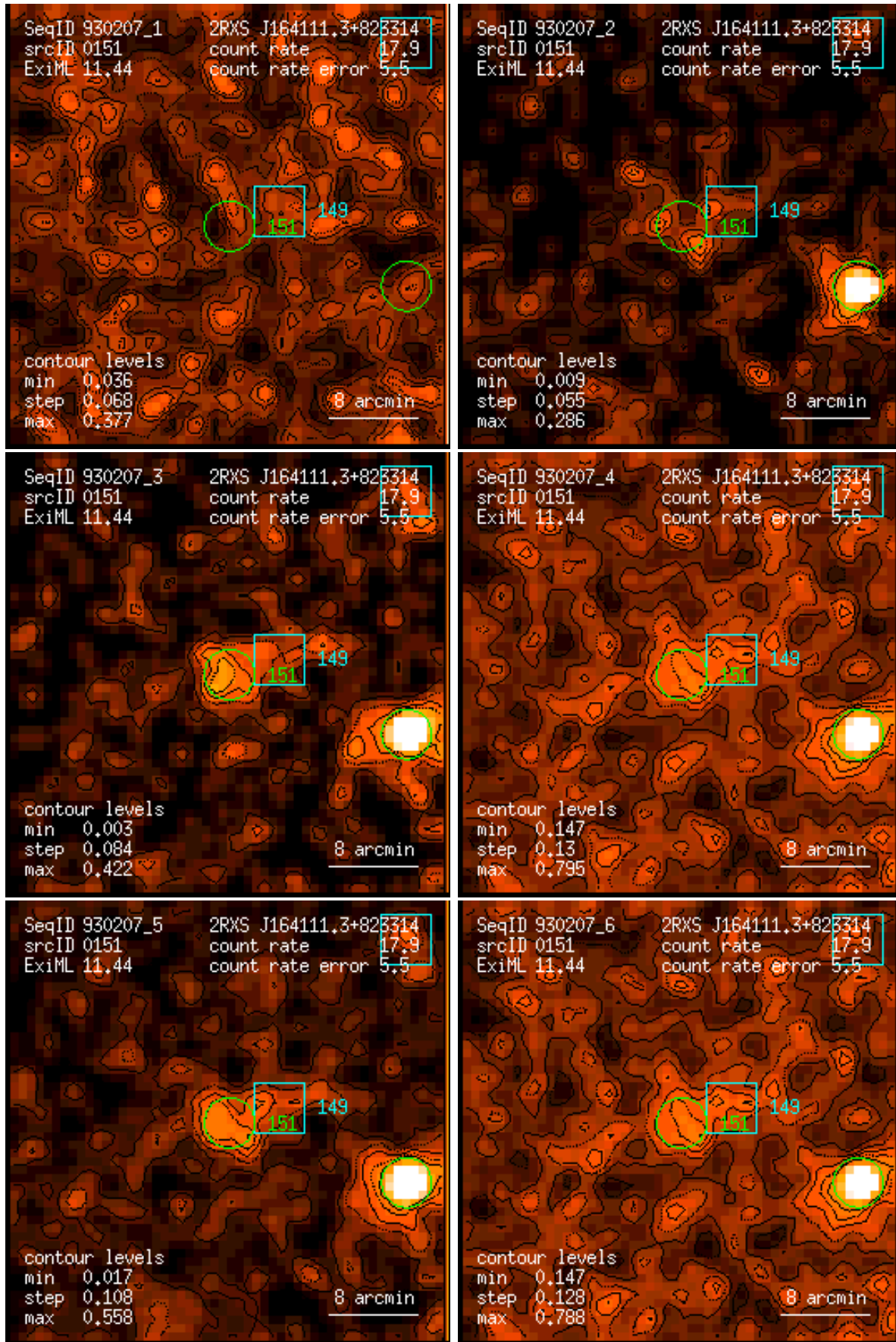
Figure 151: RASS 930207: detection 0151: band rate images, Gaussian filter: (1) PSPC channels 11 – 41, (2) 52 – 90, (3) 91 – 201, (4) 11 – 235, (5) 52 – 201, (6) 11 – 201. Broad band rates in counts/ks. Band rate contour levels in counts/ks/arcmin 2 .
