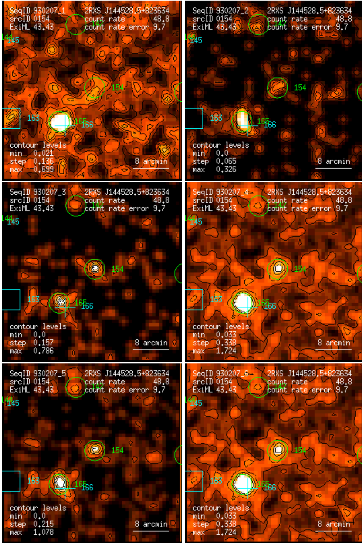
Figure 154: RASS 930207: detection 0154: band rate images, Gaussian filter: (1) PSPC channels 11 – 41, (2) 52 – 90, (3) 91 – 201, (4) 11 – 235, (5) 52 – 201, (6) 11 – 201. Broad band rates in counts/ks. Band rate contour levels in counts/ks/arcmin 2 .
