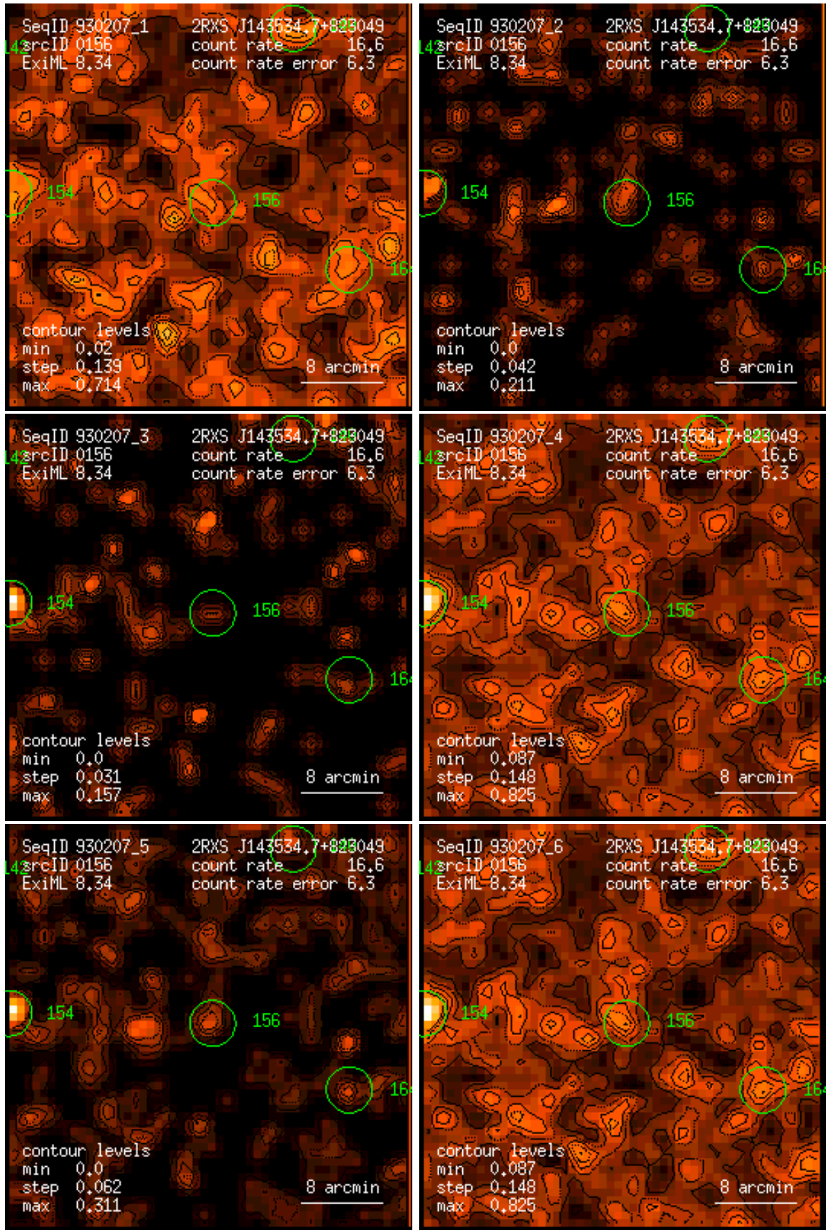
Figure 156: RASS 930207: detection 0156: band rate images, Gaussian filter: (1) PSPC channels 11 – 41, (2) 52 – 90, (3) 91 – 201, (4) 11 – 235, (5) 52 – 201, (6) 11 – 201. Broad band rates in counts/ks. Band rate contour levels in counts/ks/arcmin 2 .
