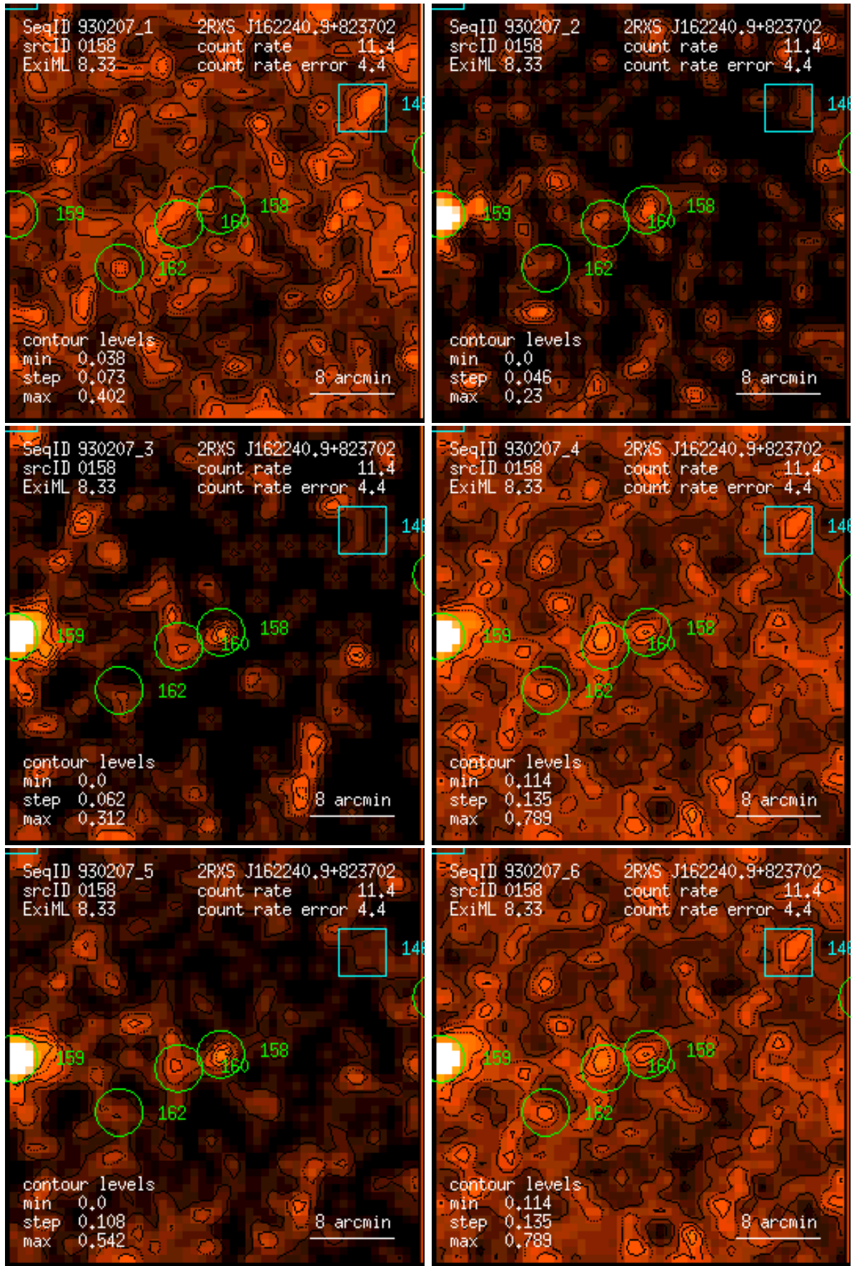
Figure 158: RASS 930207: detection 0158: band rate images, Gaussian filter: (1) PSPC channels 11 – 41, (2) 52 – 90, (3) 91 – 201, (4) 11 – 235, (5) 52 – 201, (6) 11 – 201. Broad band rates in counts/ks. Band rate contour levels in counts/ks/arcmin 2 .
