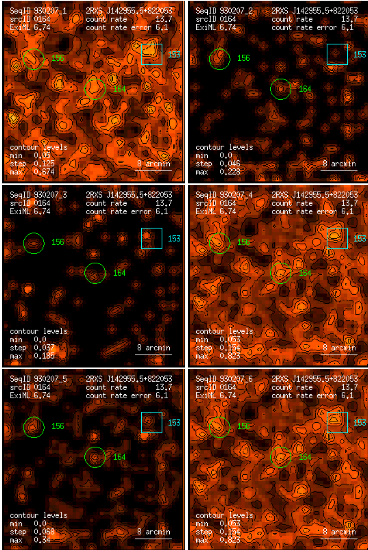
Figure 164: RASS 930207: detection 0164: band rate images, Gaussian filter: (1) PSPC channels 11 – 41, (2) 52 – 90, (3) 91 – 201, (4) 11 – 235, (5) 52 – 201, (6) 11 – 201. Broad band rates in counts/ks. Band rate contour levels in counts/ks/arcmin 2 .
