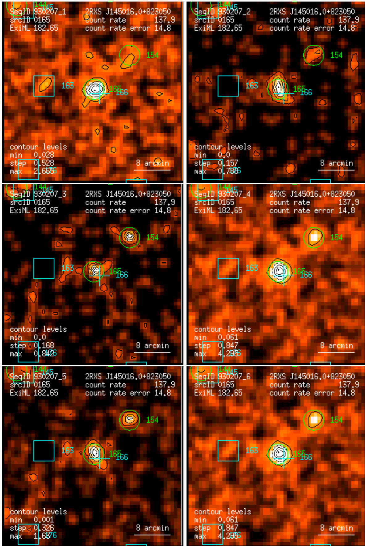
Figure 165: RASS 930207: detection 0165: band rate images, Gaussian filter: (1) PSPC channels 11 – 41, (2) 52 – 90, (3) 91 – 201, (4) 11 – 235, (5) 52 – 201, (6) 11 – 201. Broad band rates in counts/ks. Band rate contour levels in counts/ks/arcmin 2 .
