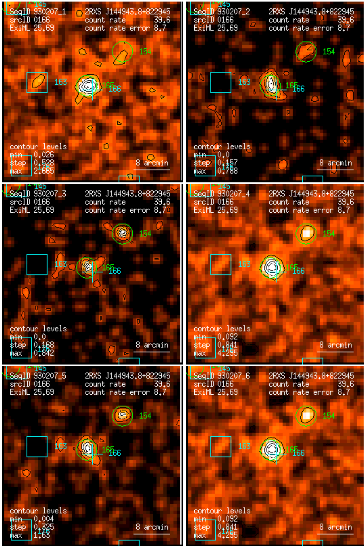
Figure 166: RASS 930207: detection 0166: band rate images, Gaussian filter: (1) PSPC channels 11 – 41, (2) 52 – 90, (3) 91 – 201, (4) 11 – 235, (5) 52 – 201, (6) 11 – 201. Broad band rates in counts/ks. Band rate contour levels in counts/ks/arcmin 2 .
