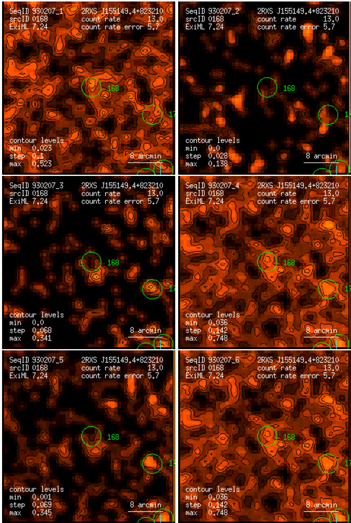
Figure 168: RASS 930207: detection 0168: band rate images, Gaussian filter: (1) PSPC channels 11 – 41, (2) 52 – 90, (3) 91 – 201, (4) 11 – 235, (5) 52 – 201, (6) 11 – 201. Broad band rates in counts/ks. Band rate contour levels in counts/ks/arcmin 2 .
