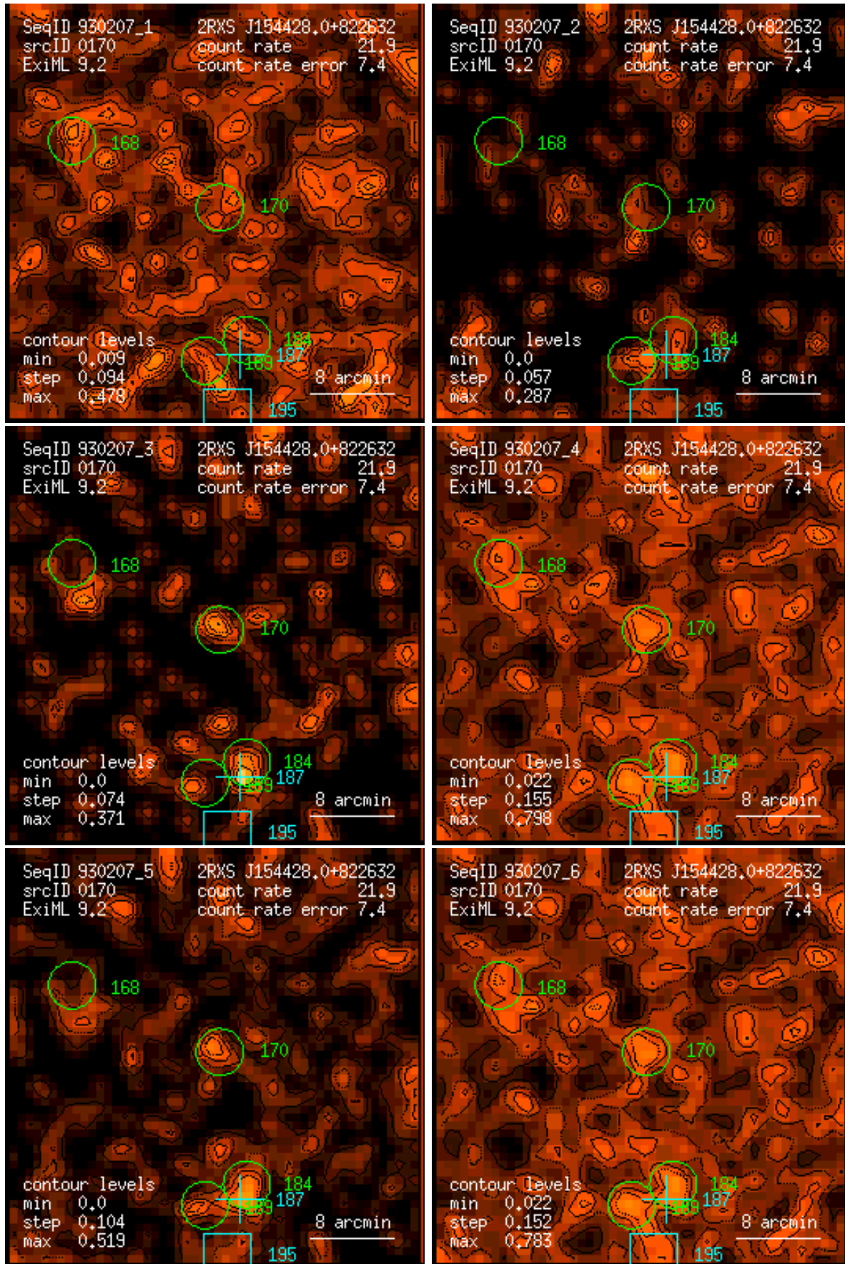
Figure 170: RASS 930207: detection 0170: band rate images, Gaussian filter: (1) PSPC channels 11 – 41, (2) 52 – 90, (3) 91 – 201, (4) 11 – 235, (5) 52 – 201, (6) 11 – 201. Broad band rates in counts/ks. Band rate contour levels in counts/ks/arcmin 2 .
