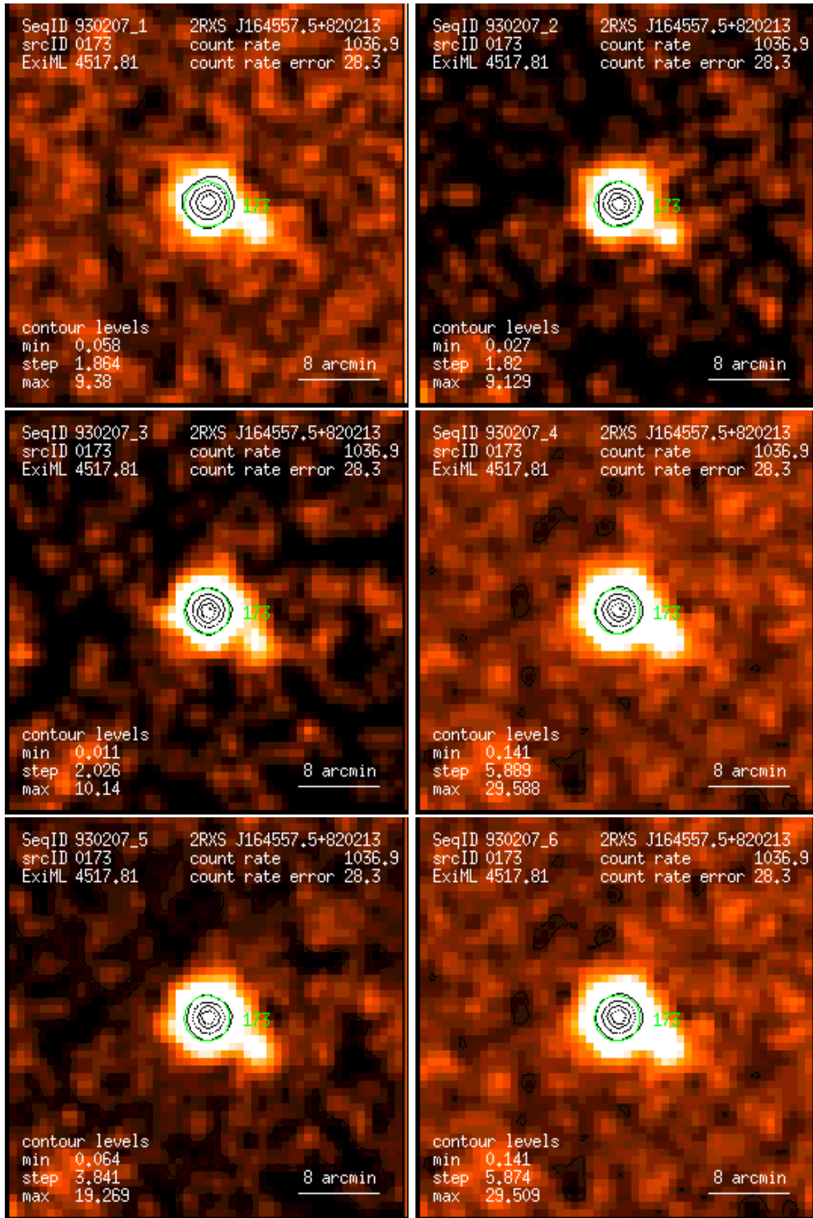
Figure 173: RASS 930207: detection 0173: band rate images, Gaussian filter: (1) PSPC channels 11 – 41, (2) 52 – 90, (3) 91 – 201, (4) 11 – 235, (5) 52 – 201, (6) 11 – 201. Broad band rates in counts/ks. Band rate contour levels in counts/ks/arcmin 2 .
