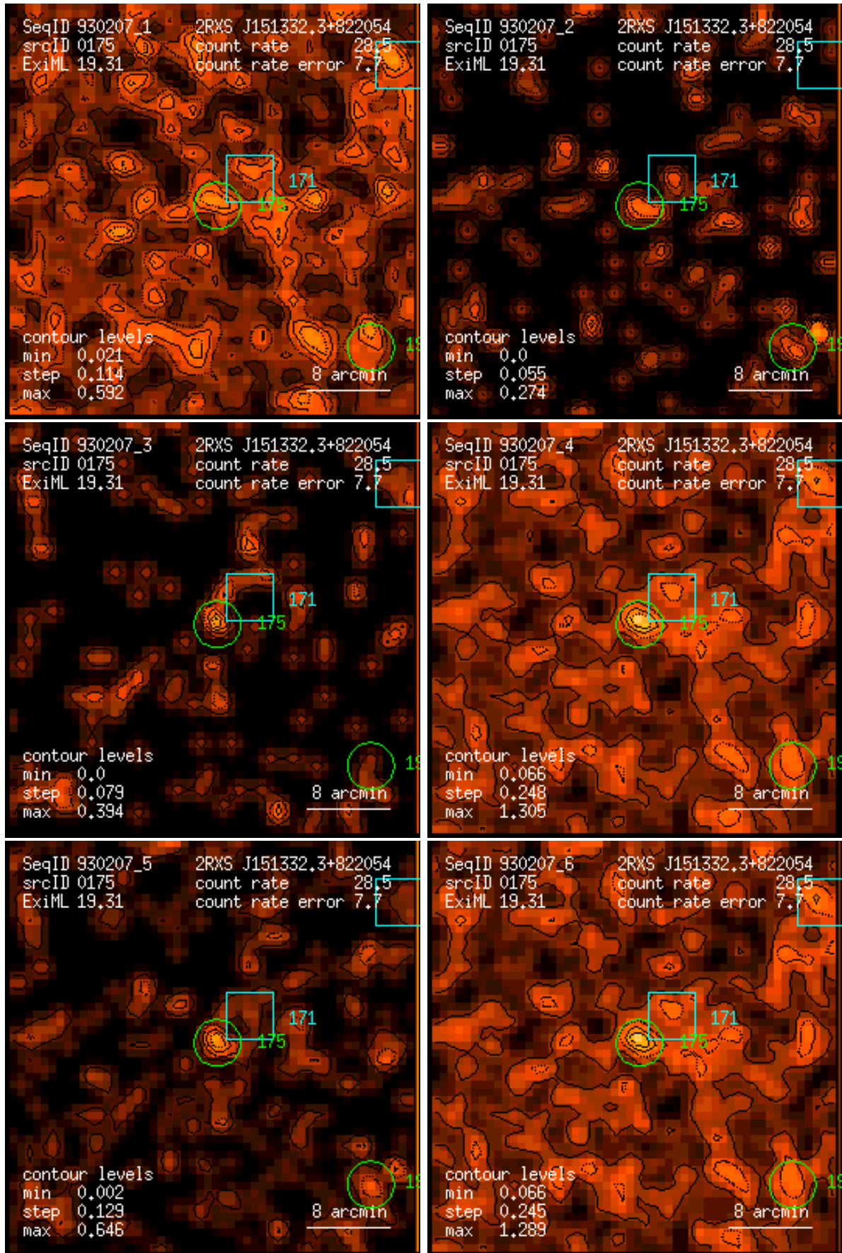
Figure 175: RASS 930207: detection 0175: band rate images, Gaussian filter: (1) PSPC channels 11 – 41, (2) 52 – 90, (3) 91 – 201, (4) 11 – 235, (5) 52 – 201, (6) 11 – 201. Broad band rates in counts/ks. Band rate contour levels in counts/ks/arcmin 2 .
