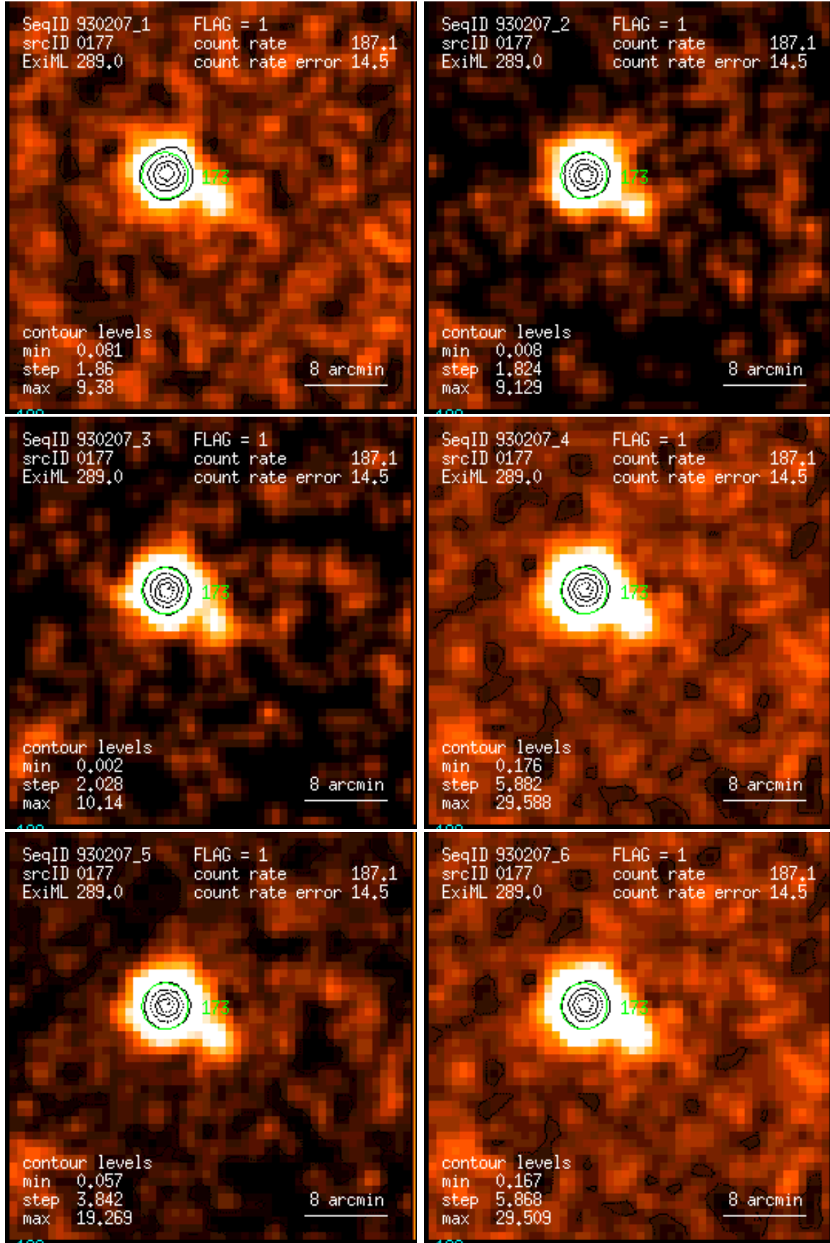
Figure 177: RASS 930207: detection 0177: band rate images, Gaussian filter: (1) PSPC channels 11 – 41, (2) 52 – 90, (3) 91 – 201, (4) 11 – 235, (5) 52 – 201, (6) 11 – 201. Broad band rates in counts/ks. Band rate contour levels in counts/ks/arcmin 2 .
