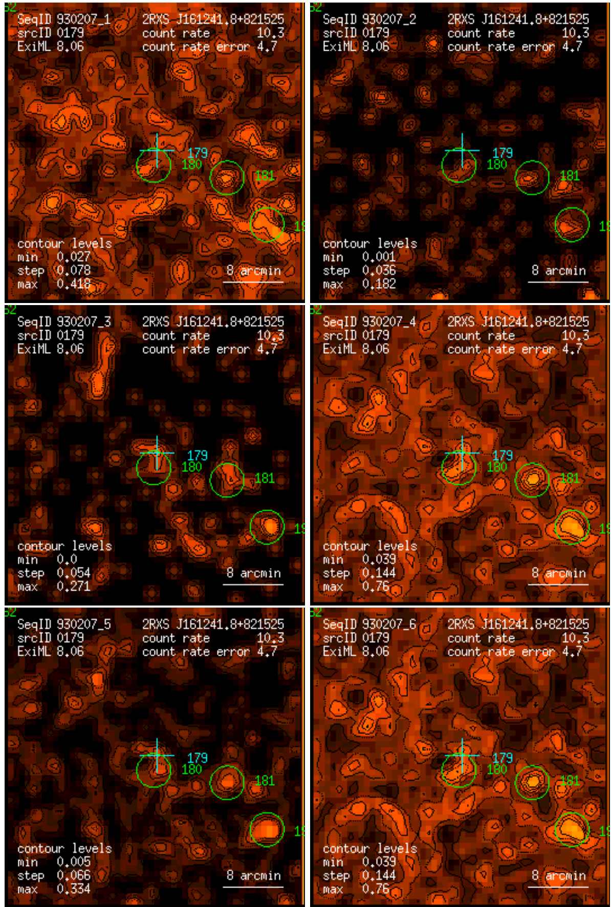
Figure 179: RASS 930207: detection 0179: band rate images, Gaussian filter: (1) PSPC channels 11 – 41, (2) 52 – 90, (3) 91 – 201, (4) 11 – 235, (5) 52 – 201, (6) 11 – 201. Broad band rates in counts/ks. Band rate contour levels in counts/ks/arcmin 2 .
