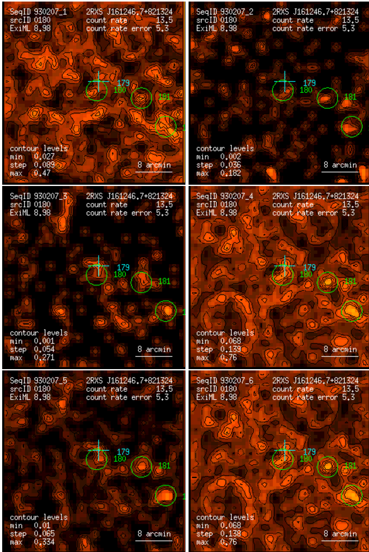
Figure 180: RASS 930207: detection 0180: band rate images, Gaussian filter: (1) PSPC channels 11 – 41, (2) 52 – 90, (3) 91 – 201, (4) 11 – 235, (5) 52 – 201, (6) 11 – 201. Broad band rates in counts/ks. Band rate contour levels in counts/ks/arcmin 2 .
