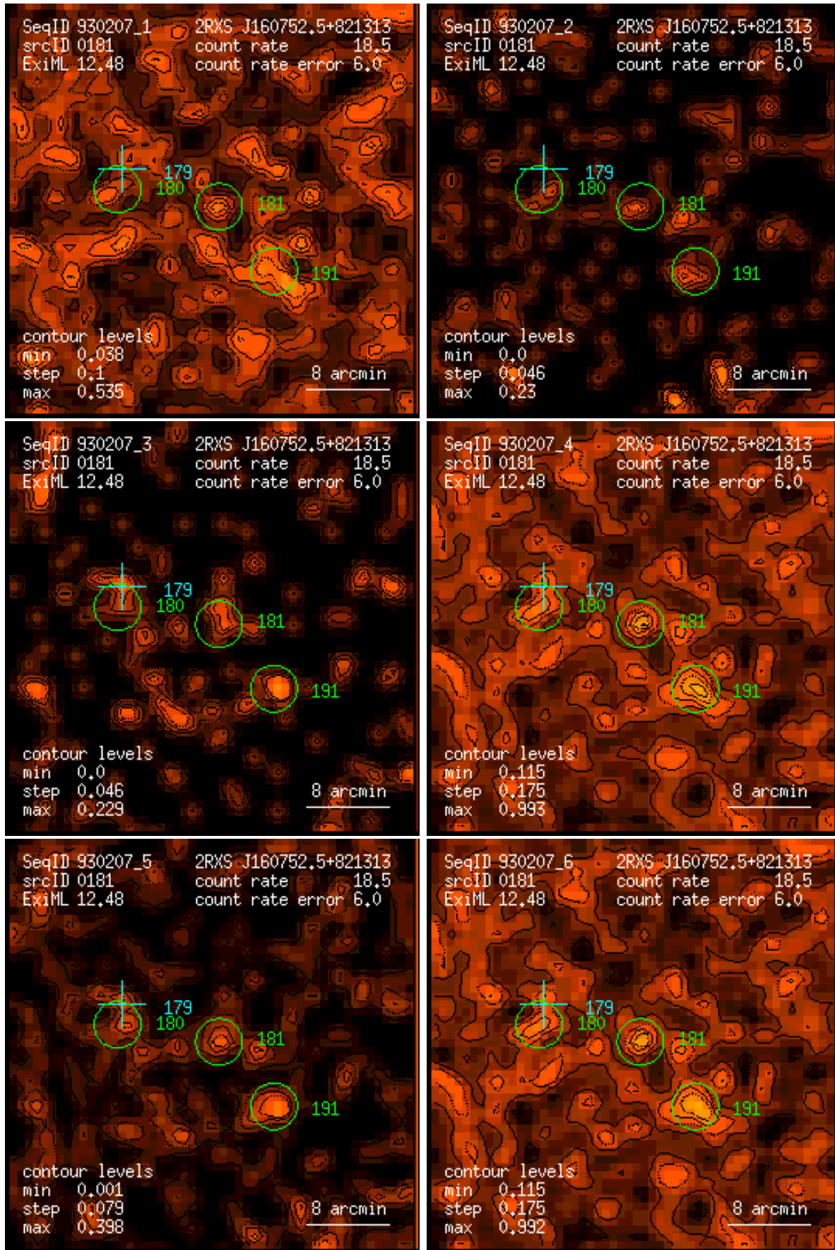
Figure 181: RASS 930207: detection 0181: band rate images, Gaussian filter: (1) PSPC channels 11 – 41, (2) 52 – 90, (3) 91 – 201, (4) 11 – 235, (5) 52 – 201, (6) 11 – 201. Broad band rates in counts/ks. Band rate contour levels in counts/ks/arcmin 2 .
