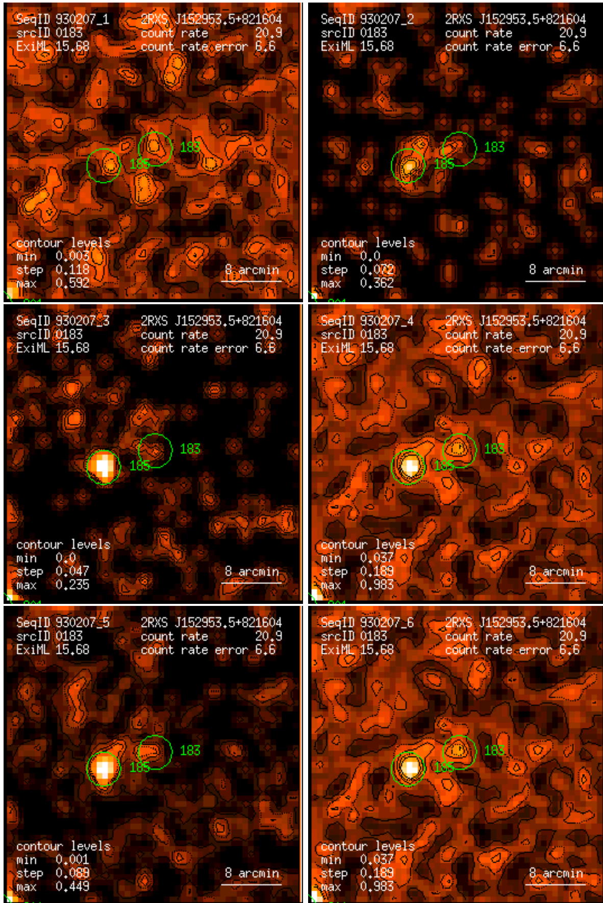
Figure 183: RASS 930207: detection 0183: band rate images, Gaussian filter: (1) PSPC channels 11 – 41, (2) 52 – 90, (3) 91 – 201, (4) 11 – 235, (5) 52 – 201, (6) 11 – 201. Broad band rates in counts/ks. Band rate contour levels in counts/ks/arcmin 2 .
